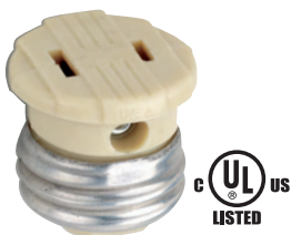
90-546 Ivory 80-2513 White Medium Base - Polarized Socket Outlet Adapter 660W-125V
