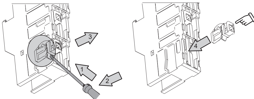
Figure 5-6 Deinstalling the slider from the terminal module
