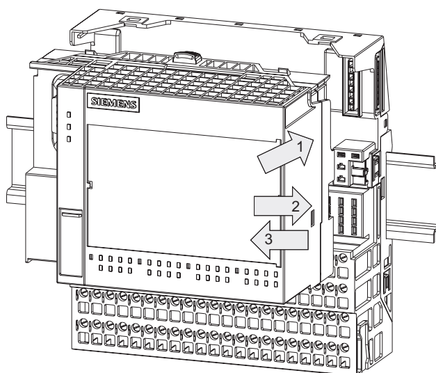
Figure 5-13 Inserting and identifying a COMPACT module
