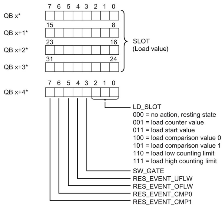
Figure 4-3 Assignment of the control interface
