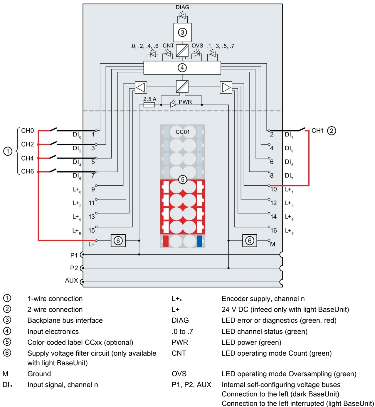
Figure 5-1 Pinout and block diagram for 1 and 2-wire connection of encoders
