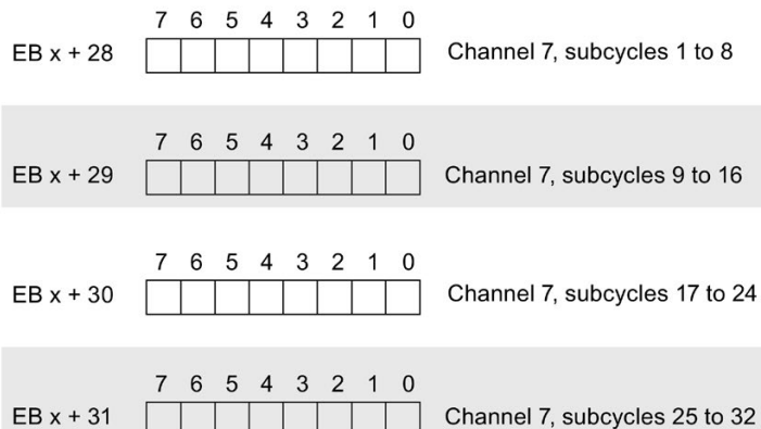
Figure 5-5 Address space for oversampling
