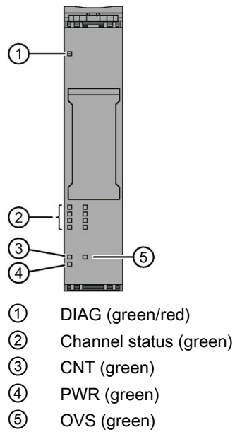
Figure 4-6 LED display
