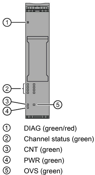
Figure 5-6 LED display
