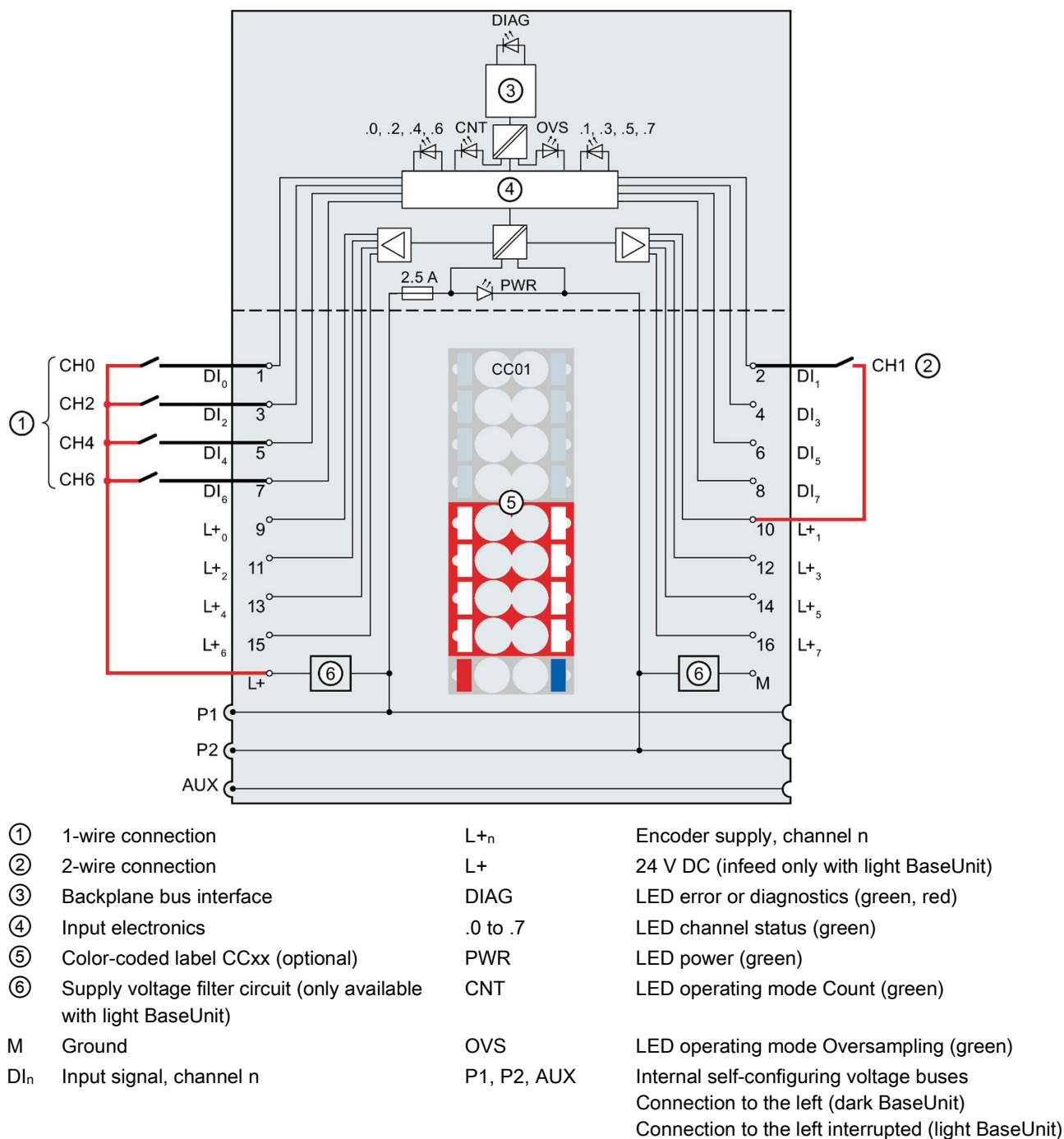
Figure 3-1 Pinout and block diagram for 1 and 2-wire connection of encoders
