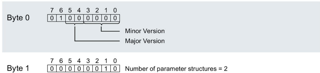
Figure A-14 Structure of the header information
