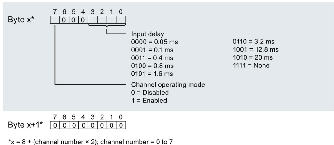
Figure A-18 Structure byte x to x+1 for the channels 0 to 7
