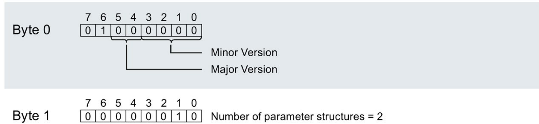
Figure A-2 Structure of the header information
