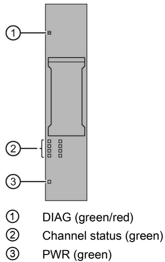
Figure 5-1 LED display
