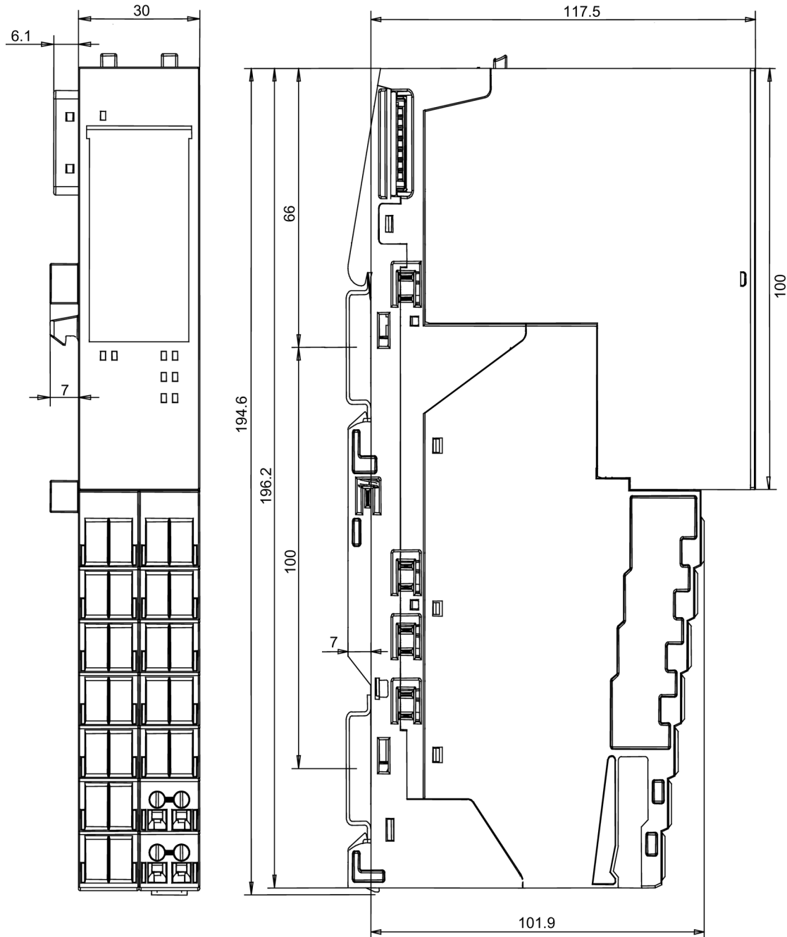
Figure B-2 Dimension drawing of terminal module with PM-D F DC24V PROFIsafe
