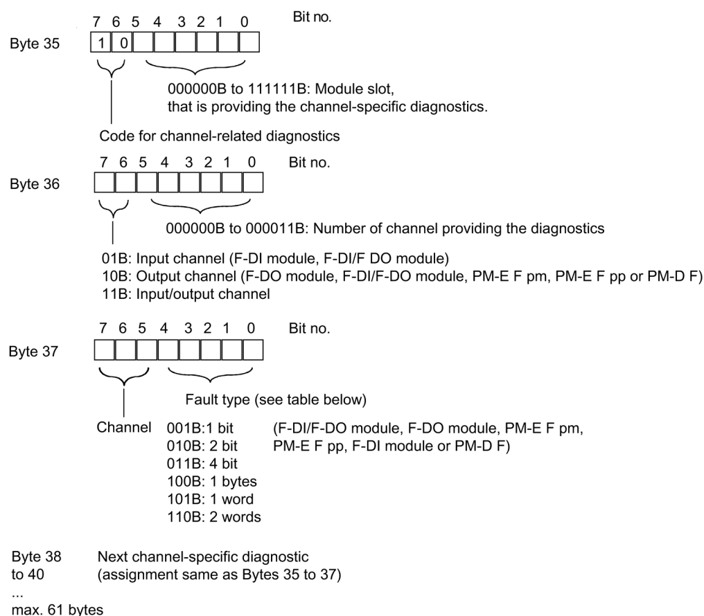
Figure 5-1 Structure of Channel-specific diagnostics
