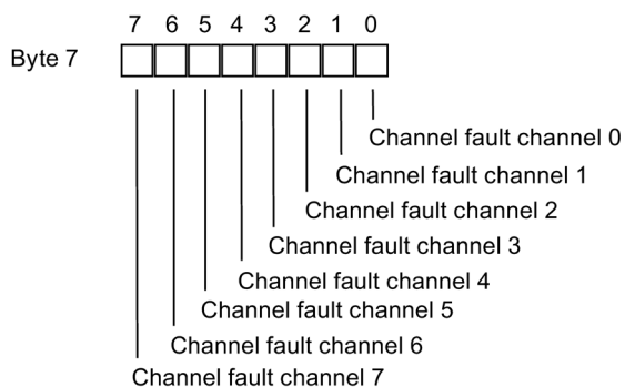
Figure A-4 Byte 7 of diagnostics data for EM 4/8 F-DI DC24V PROFIsafe
