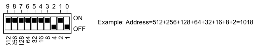
Figure 3-1 Example for Setting the Address Switch (DIP Switch)
