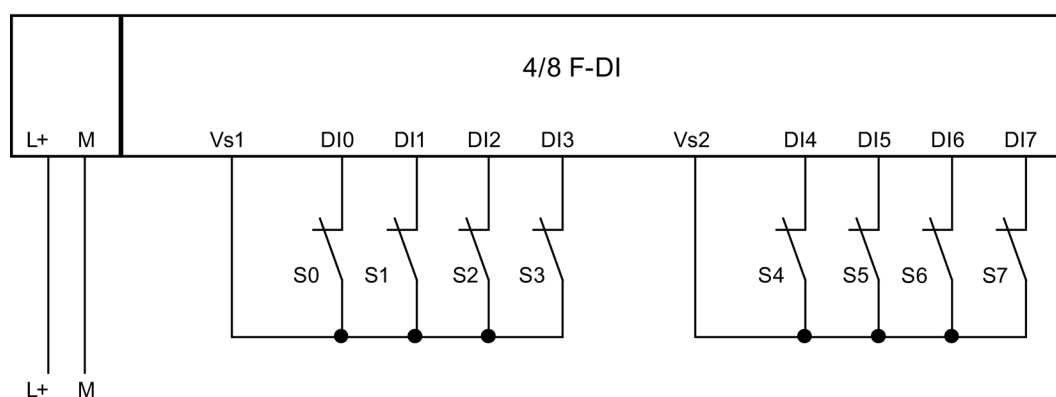
Figure 7-19 Wiring diagram EM 4/8 F-DI DC24V PROFIsafe - one sensor connected via one channel, internal sensor supply
