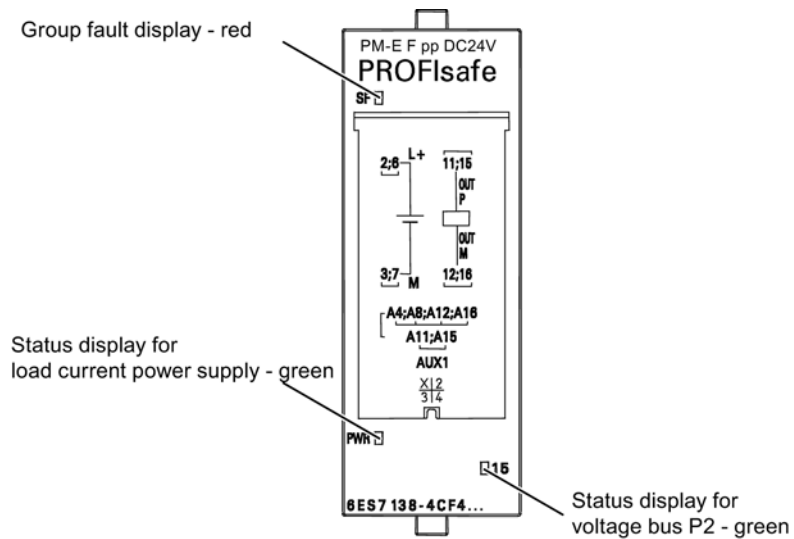
Figure 7-9 Front view PM-E F pp DC24V PROFIsafe
