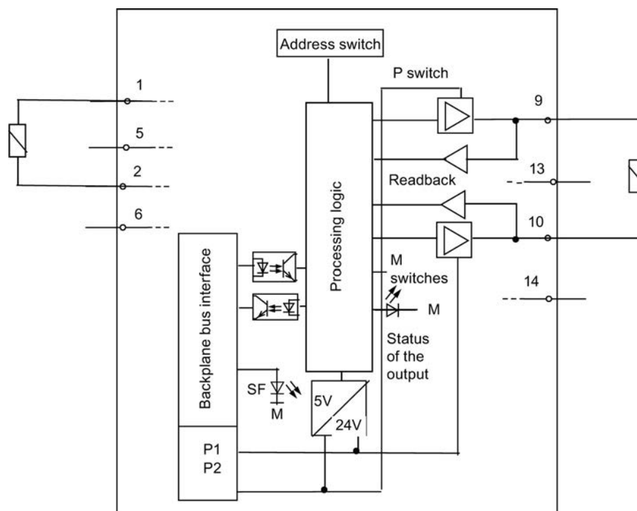
Figure 7-50 Block diagram of the EM 4 F-DO DC24V/2A PROFIsafe
