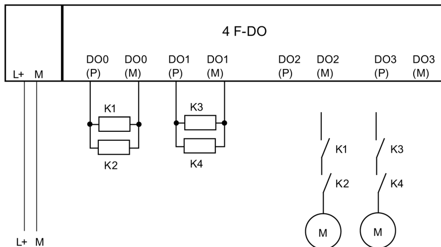
Figure 7-53 Wiring diagram for in each case 2 relays parallel on 1 F-DO of the EM 4 F-DO DC24V/2A PROFIsafe
