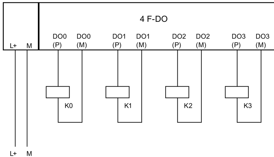
Figure 7-51 Wiring diagram of the EM 4 F-DO DC24V/2A PROFIsafe
