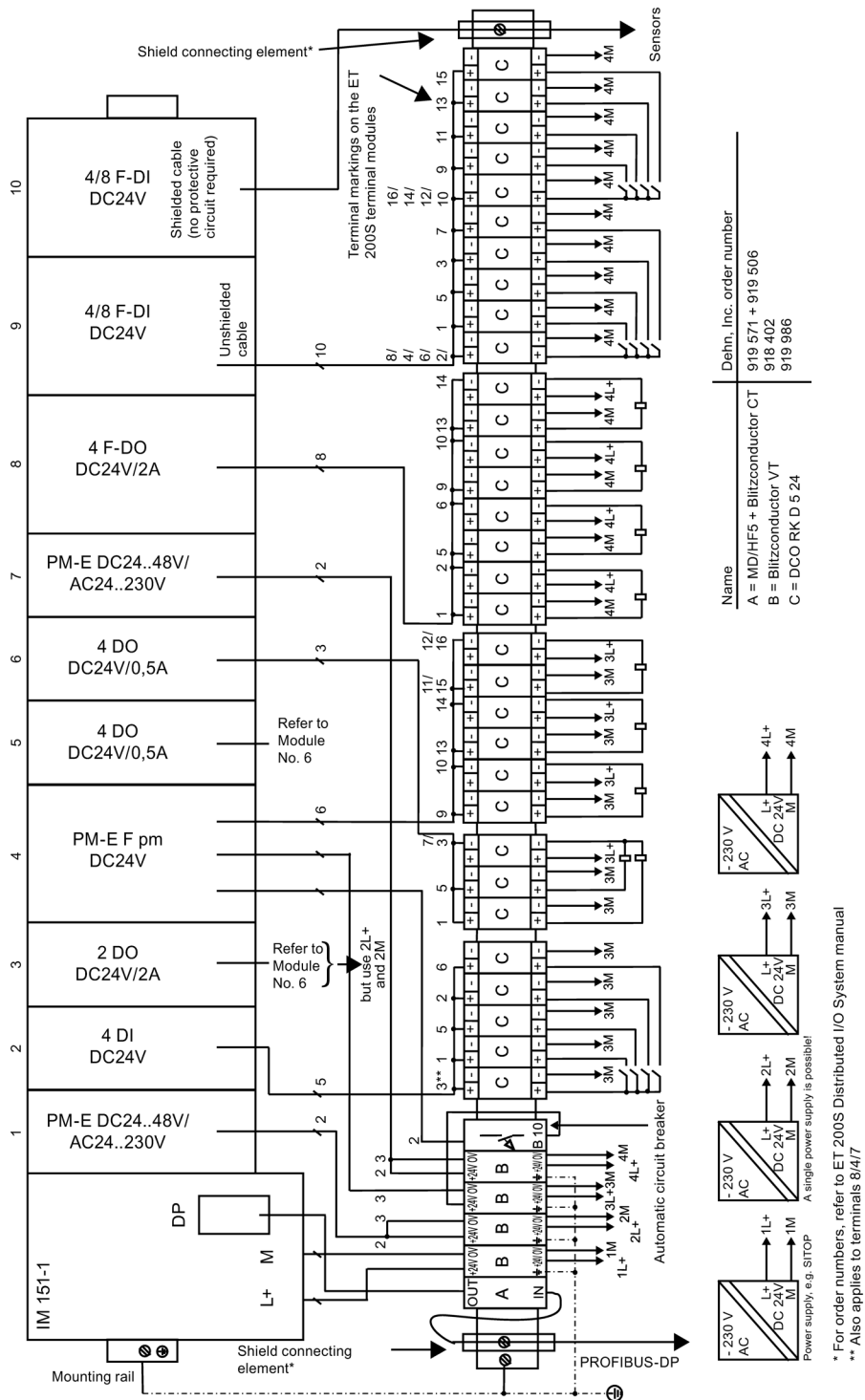
Figure 6-1 External Protective Circuit (Surge Filter) for ET 200S with Fail-Safe Modules
