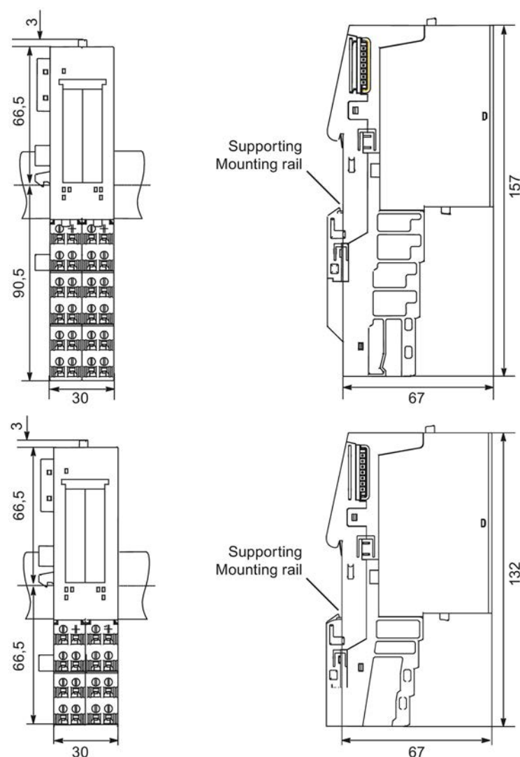
Figure B-1 Dimension Drawing of Terminal Modules with PM-E F pm, PM-E F pp, F-DI or F-DO module
