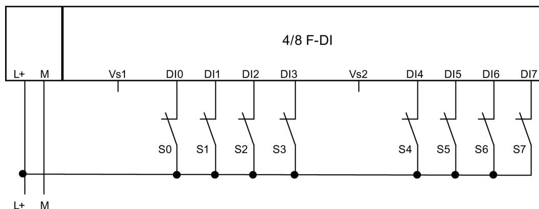
Figure 7-20 Wiring diagram EM 4/8 F-DI DC24V PROFIsafe - one sensor connected via one channel, internal sensor supply
