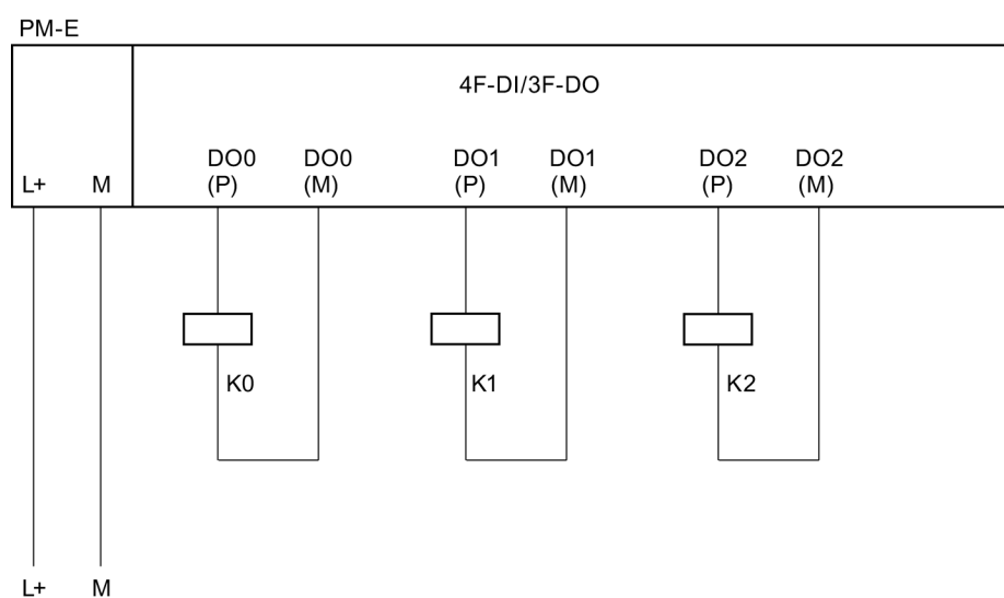
Figure 7-45 Wiring Diagram EM 4 F-DI/3 F-DO DC24V - Output Circuit
