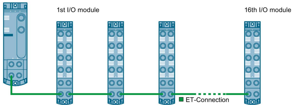
Figure 3-1 ET 200AL with ET-Connection1
