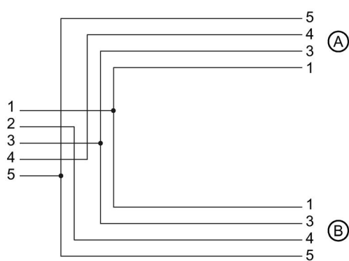
Figure 5-10 Wiring of the Y-cable
