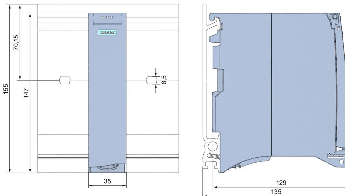
Figure A-1 Dimensional drawing of the IM 155-5 PN ST interface module, front and side views
