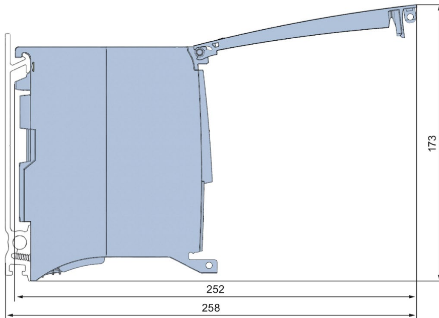
Figure A-2 Dimensional drawing of the IM 155-5 PN ST interface module, side view with open front cover
