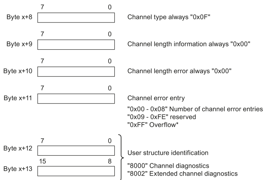
Figure 4-8 Structure starting at byte x+8
