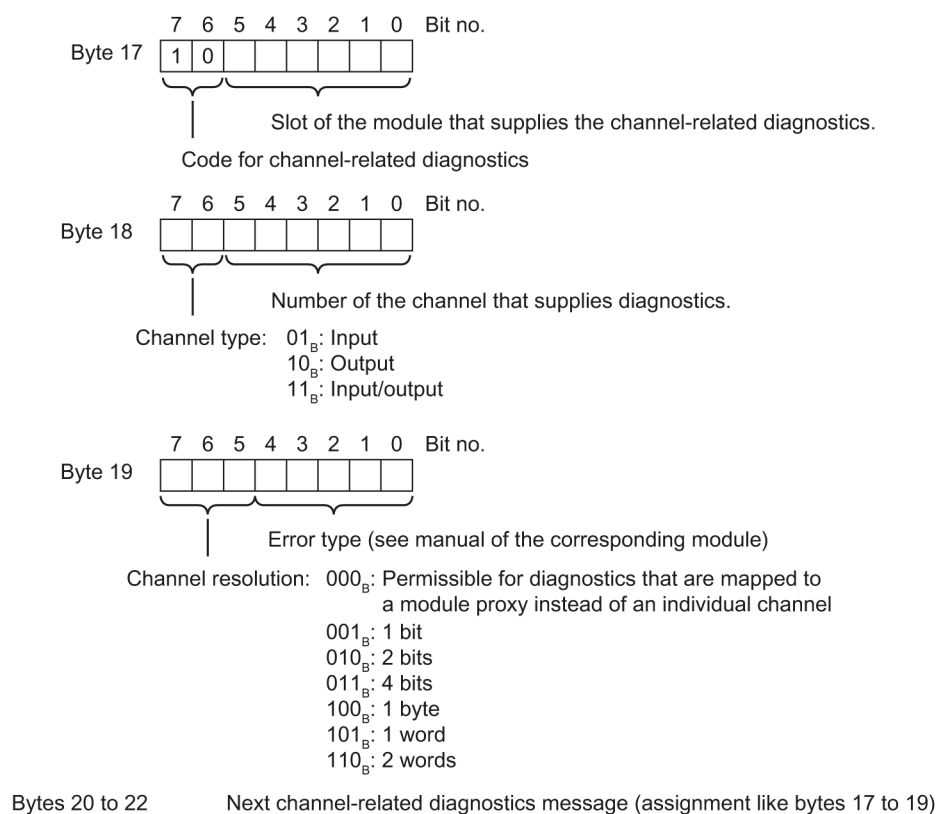
Figure 4-5 Structure of the channel diagnostics
