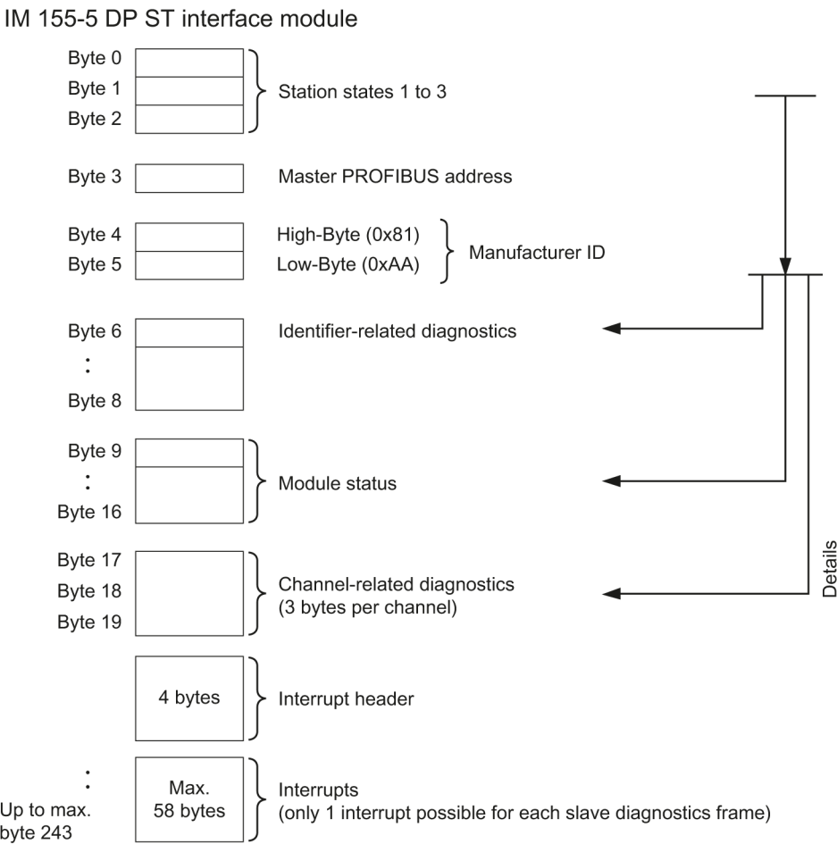
Figure 4-2 Configuration of the slave diagnostics DP
