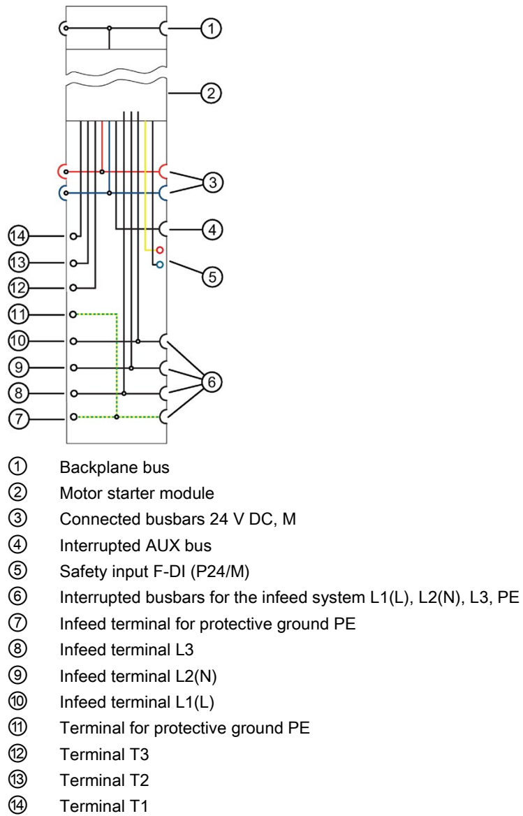
Figure 5-10 BaseUnit block diagram with 500 V AC infeed and fail-safe input
