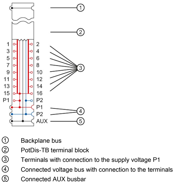
Figure 6-4 Block diagram of the PotDis-BU type P1, dark-colored version
