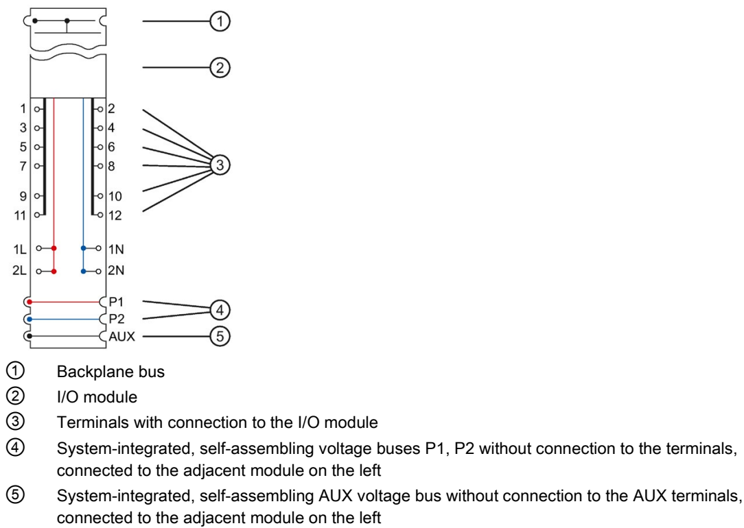
Figure 4-20 Block diagram of the BU type B1, dark-colored version, without AUX terminals, supply over supply terminals
