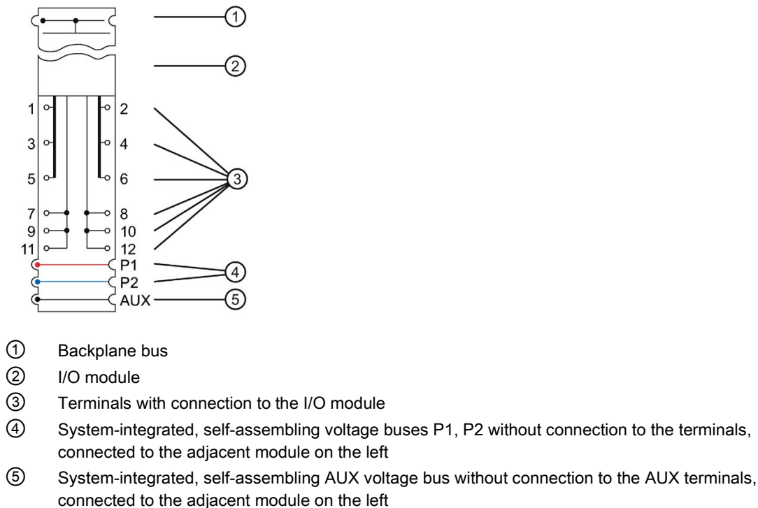
Figure 4-26 Block diagram of the BU type D0, dark-colored version, without AUX terminals, supply over supply terminals
