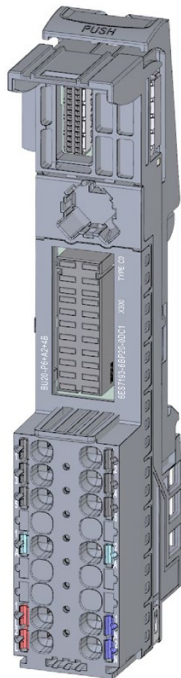
Figure 4-23 BU type C1, dark-colored version, with AUX terminals, supply over P1, P2 busbar
