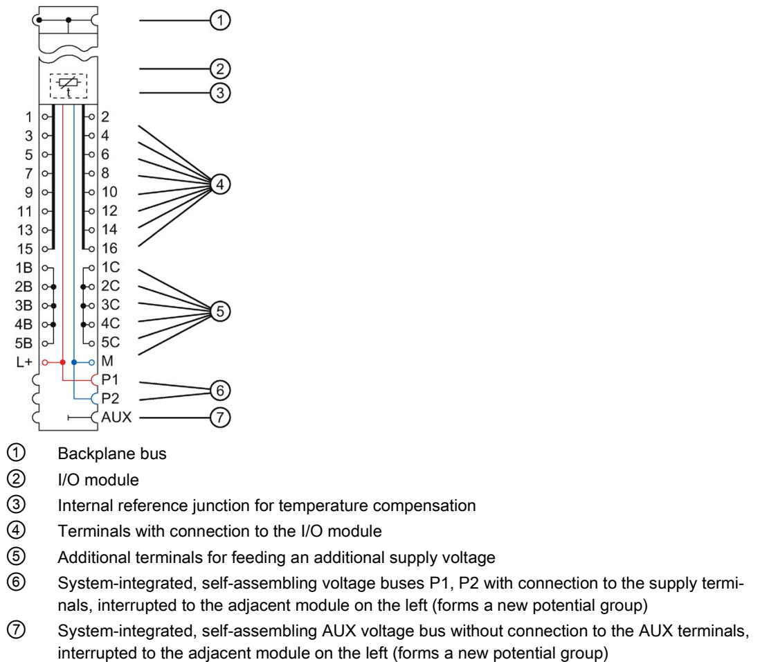
Figure 4-10 Block diagram of the BU type A1, light-colored version, with additional terminals
