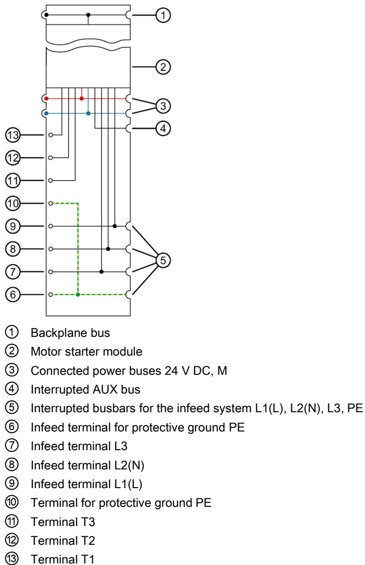
Figure 5-4 Block diagram BaseUnit with 500 V AC infeed
