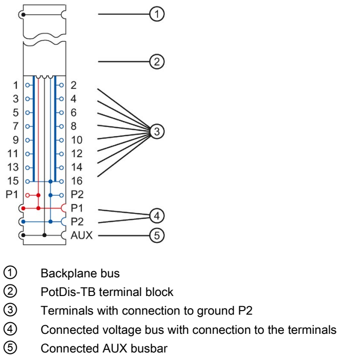
Figure 6-8 Block diagram of the PotDis-BU type P2, dark-colored version
