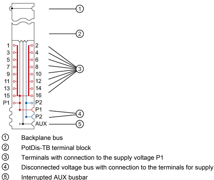
Figure 6-2 Block diagram of the PotDis-BU type P1, light-colored version
