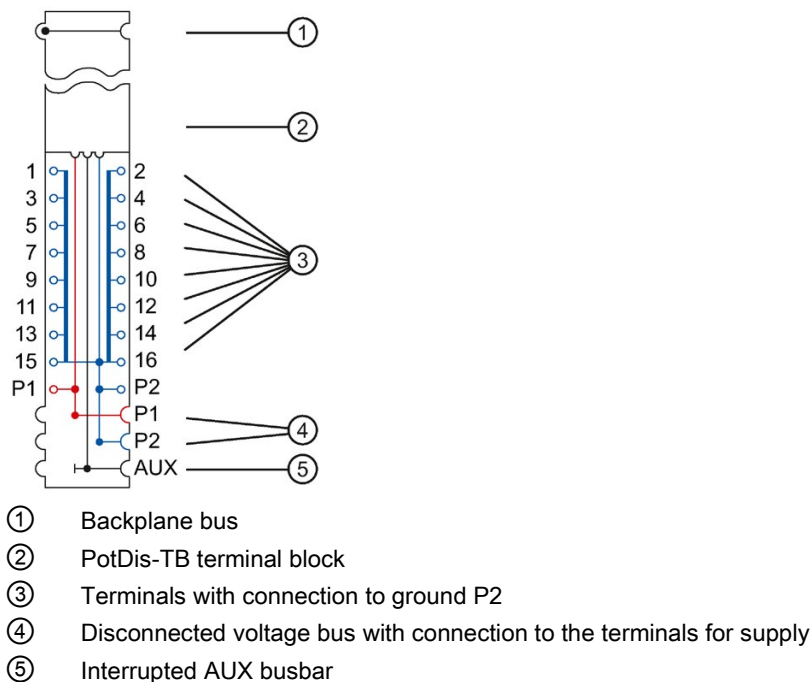
Figure 6-6 Block diagram of the PotDis-BU type P2, light-colored version
