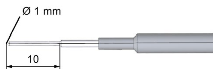
Figure A-4 Dimension drawing test probe
