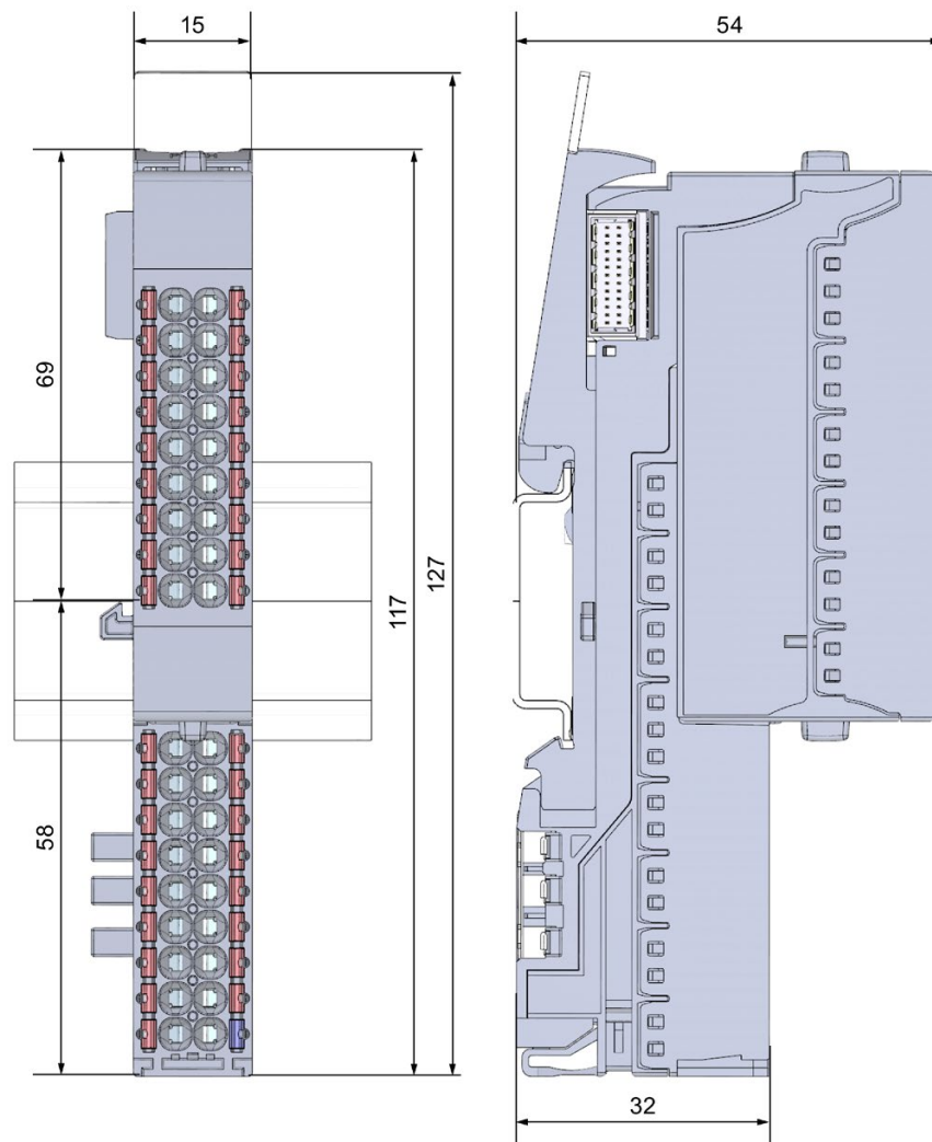
Figure 7-1 Dimension drawing of PotDis BU-P1/B-R with plugged-in terminal block
