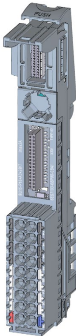
Figure 4-15 BU type A1, dark-colored version, without additional terminals
