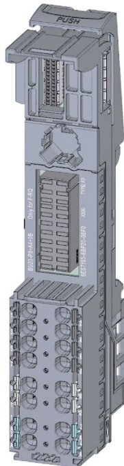
Figure 4-27 BU type F0, dark-colored version, with AUX terminals, supply over supply terminals
