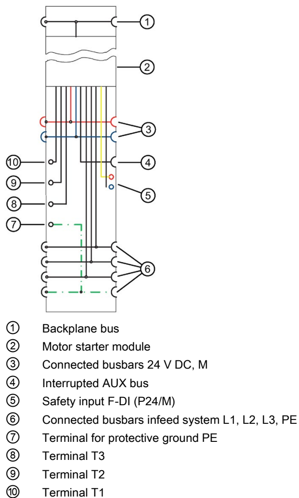
Figure 5-12 Block diagram BaseUnit without infeed, with fail-safe input
