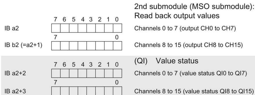
Figure 4-3 Address space for configuration as 1 x 16-channel DQ 16x24...48VUC/125VDC/0.5A ST S MSO with value status
