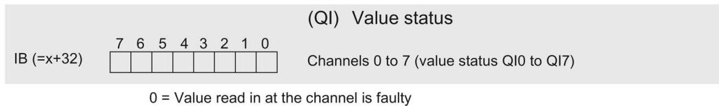
Figure 4-6 Address space for configuration as 1 x 8-channel AI 8xU/I HF MSI Scale with value status
