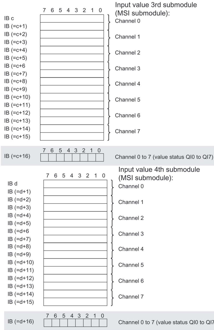
Figure 4-5 Address space for configuration as 1 x 8-channel AI 8xU/I HF MSI with value status
