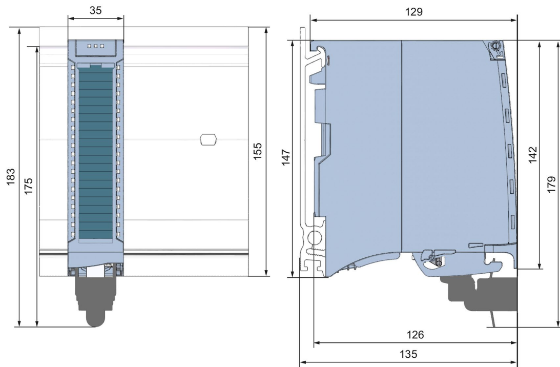
Figure A-1 Dimensional drawing of the AI 8xU/I HS module
