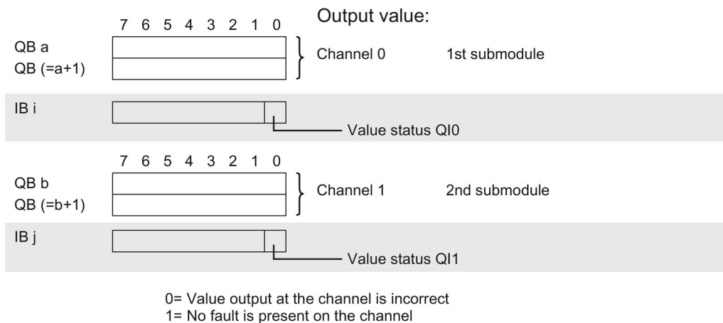
Figure 4-2 Address space for configuration as 2 x 1-channel AQ 2xU/I ST S QI with value status
