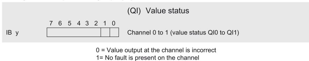
Figure 4-1 Address space for configuration as 1 x 2-channel AQ 2xU/I ST with value status
