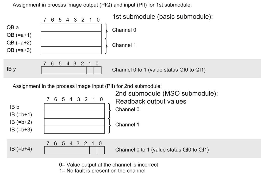
Figure 4-3 Address space for configuration as 1 x 2-channel AQ 2xU/I ST MSO with value status
