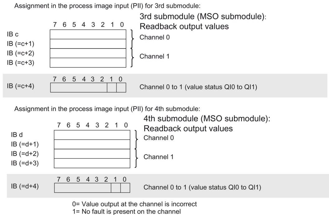
Figure 4-4 Address space for configuration as 1 x 2-channel AQ 2xU/I ST MSO with value status
