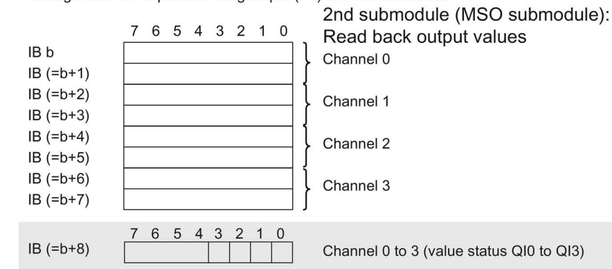
Figure 4-3 Address space for configuration as 1 x 4-channel AQ 4xU/I HF MSO with value status
