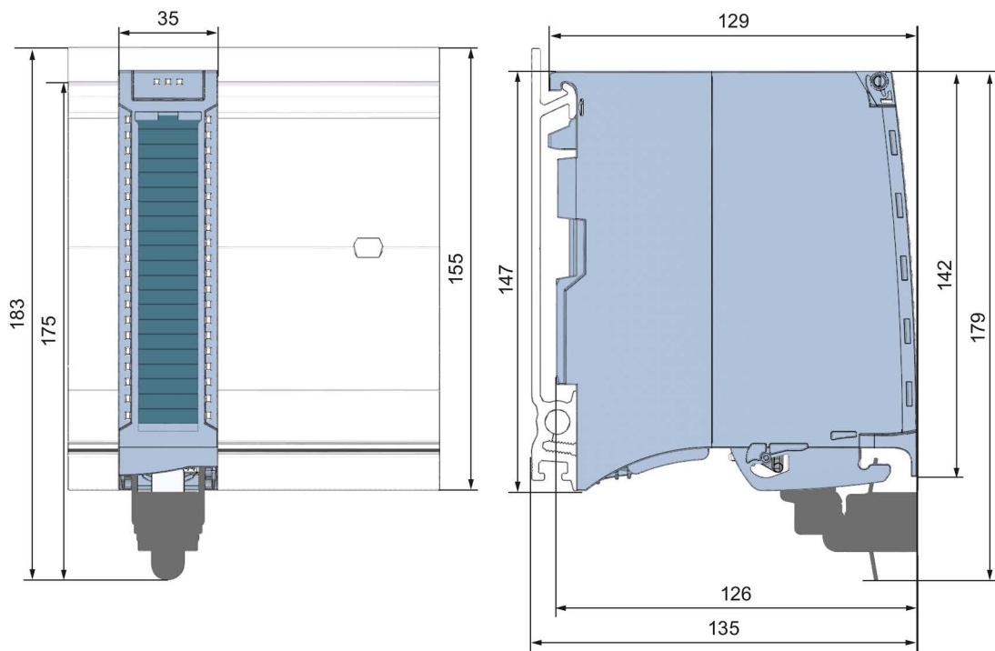
Figure A-1 Dimension drawing of the AQ 4xU/I HF module
