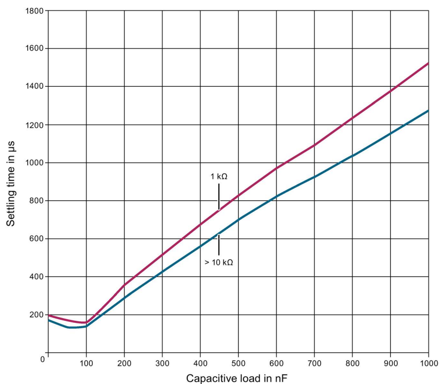
Figure 6-1 Typical settling times for voltage outputs
