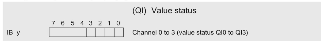
Figure 4-1 Address space for configuration as 1 x 4-channel AQ 4xU/I HF with value status
