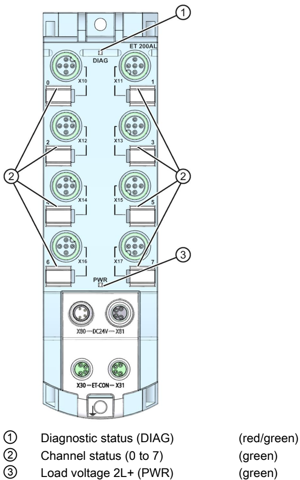
Image 5-1 LED displays
