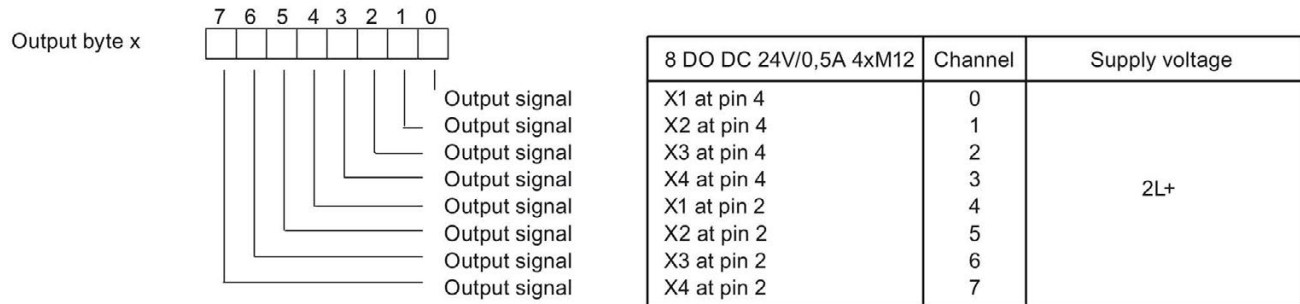
Figure E-5 Address space of 8 DO DC 24V/0,5A 4×M12 I/O device
