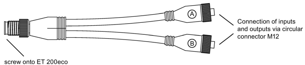
Figure 3-3 Y cable
