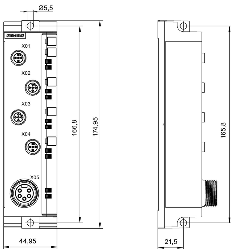
Figure 2-3 Mounting the PD DC 24V 1×7/8" 4×M12 on a panel (45 mm)
