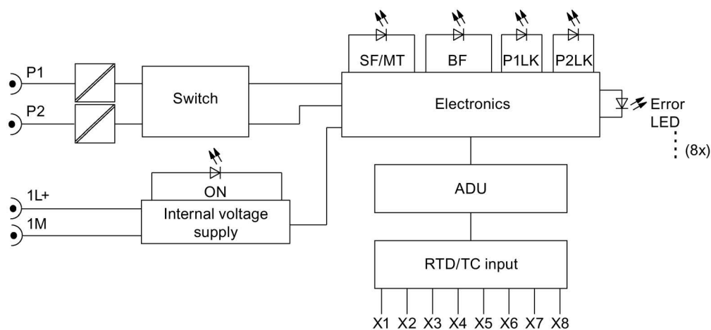
Figure 10-2 Block diagram 8 AI RTD/TC 8xM12
