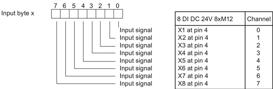
Figure E-2 Address space of 8DI DC 24V 8×M12 I/O device
