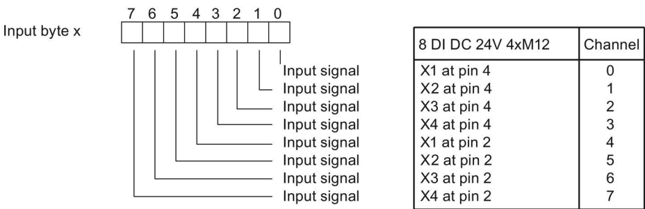
Figure E-1 Address space of 8 DI DC 24V 4×M12 I/O device
