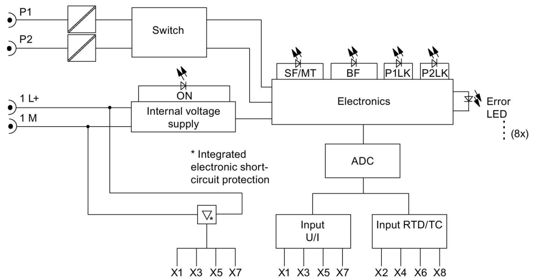
Figure 10-1 Block diagram 8 AI 4 U/I + 4 RTD/TC 8×M12
