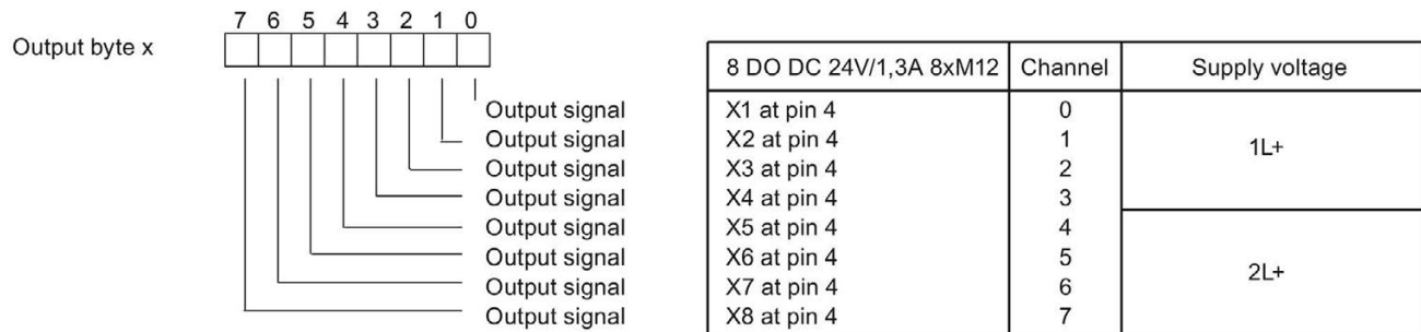
Figure E-6 Address space of I/O device 8 DO DC 24V/1,3A 8×M12 and 8 DO DC 24V/2,0A 8×M12
