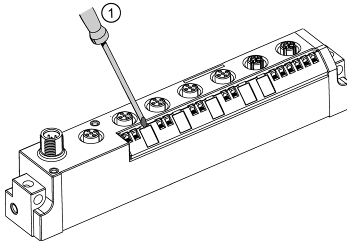
Figure 2-7 Removing labels
