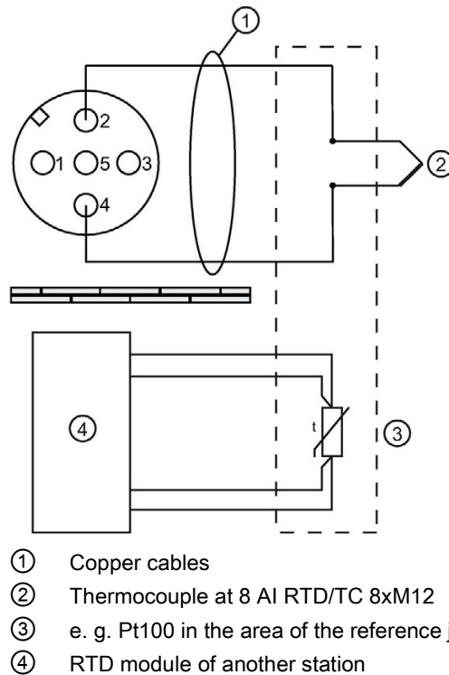
Figure D-6 Connection example "Dynamic reference temperature" as reference junction
