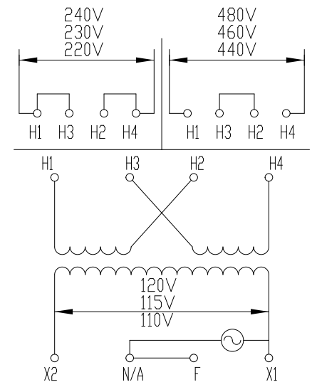
CONNECTION DIAGRAM
