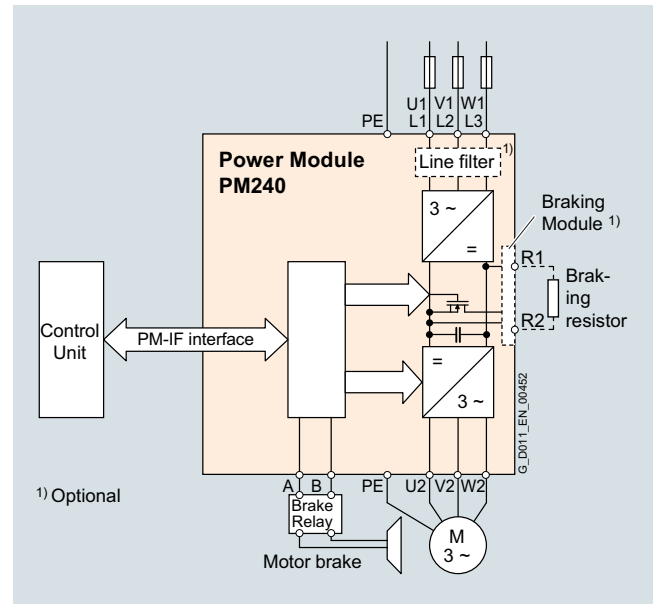
Connection example for PM240 Power Modules, frame size FSGX
