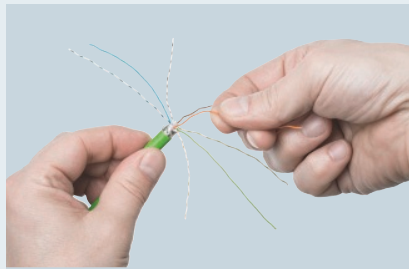
Unravel and smooth out the twisted wires
