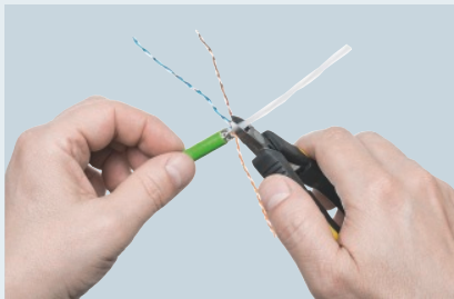
Remove the interior support cross
