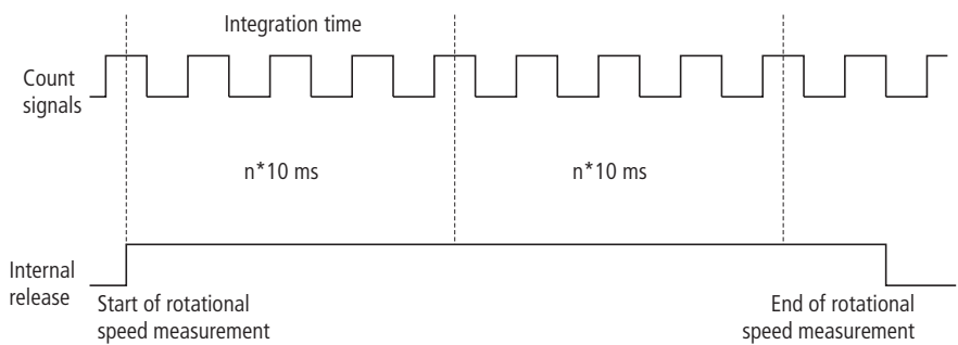
Figure 10-14: Revolutions measurement with release function
