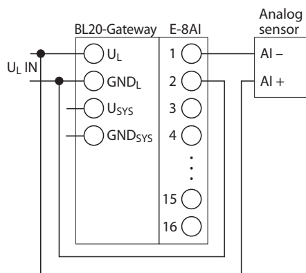
Figure 6-52: 2-wire-sensor (U/I)
