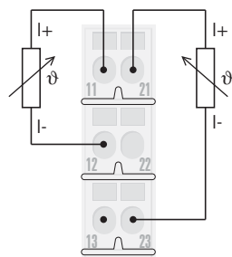
Figure 6-35: Wiring diagram BL20-S3x-SBB
