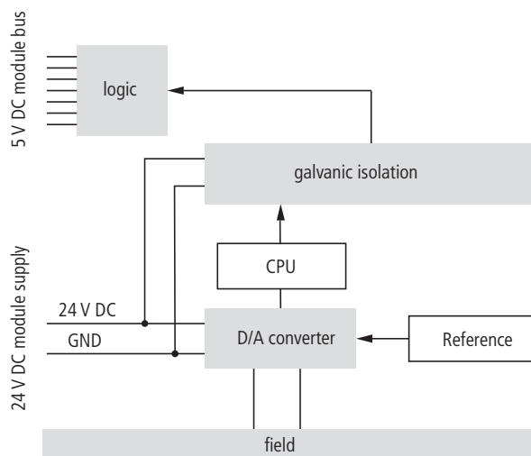
Figure 8-14: Block diagram
