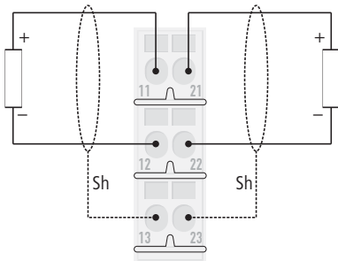
Figure 8-8: Wiring diagram BL20-S3x-SBB
