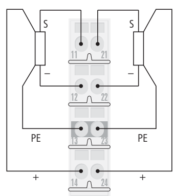
Figure 7-6: Wiring diagram BL20-S4x-SBCS
