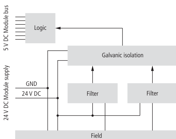
Figure 5-8: Block diagram
