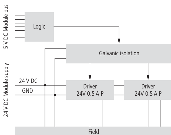
Figure 7-2: Block diagram
