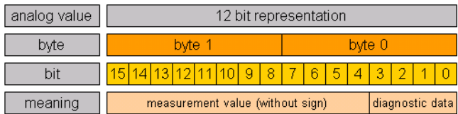
Figure 14-2: 12-bit-representation
