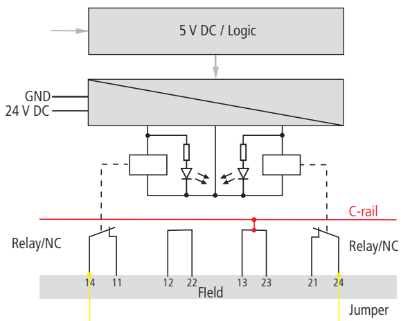
Figure 9-4: Block diagram with base module BL20-S4x-SBCS
