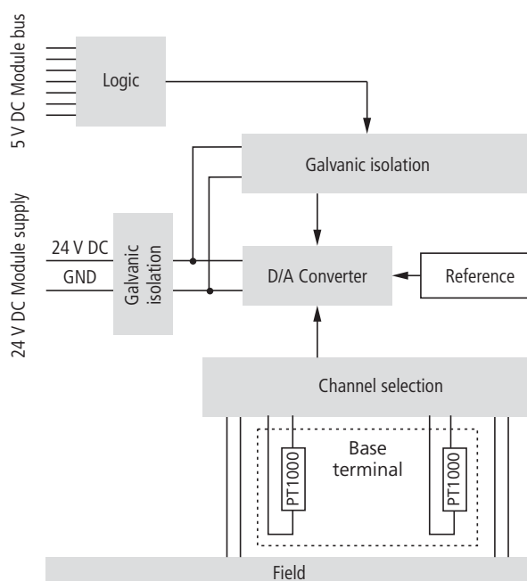
Figure 6-38: Block diagram
