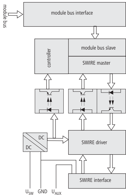
Figure 10-45: block diagram
