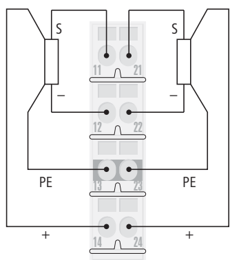
Figure 7-44: Wiring diagram BL20-S4x-SBCS
