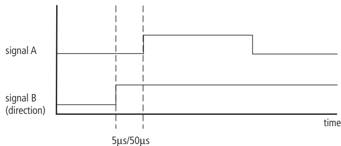
Figure 10-5: Time between direction signal and counter signal
