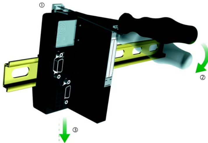
Figure 11-19: Dismounting gateway
