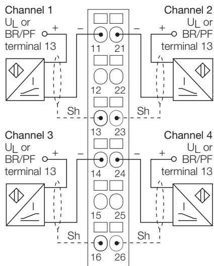
Figure 6-44: 2-wire sensors with sensor supply via UL or BR/PF- module, base module BL20-S6x-SBCSBC
