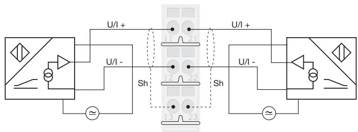
Figure 6-15: 4-wire sensor with external sensor supply BL20-S3x-SBB
