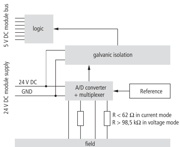
Figure 6-42: Block diagram
