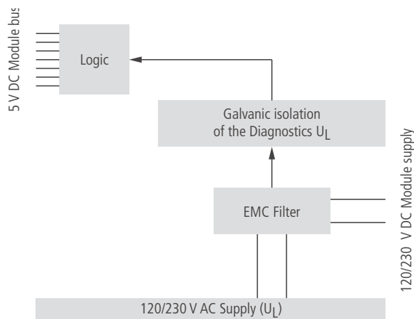
Figure 4-8: Block diagram
