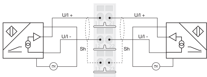
Figure 6-30: 4-wire sensor with external sensor supply BL20-S3x-SBB
