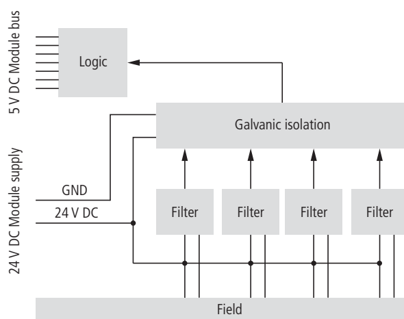
Figure 5-32: Block diagram
