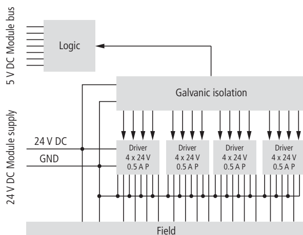
Figure 7-29: Block diagram
