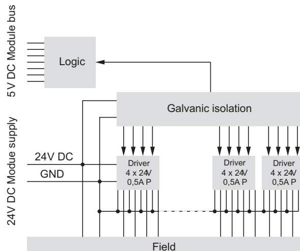
Figure 7-36: Block diagram
