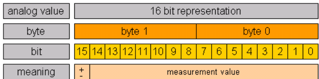
Figure 14-1: 16-bit-representation
