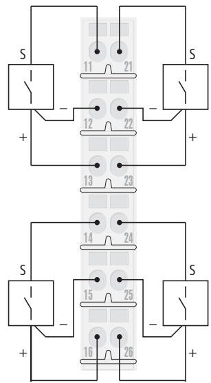
Figure 5-24: Wiring diagram BL20-S6x-SBBSBB
