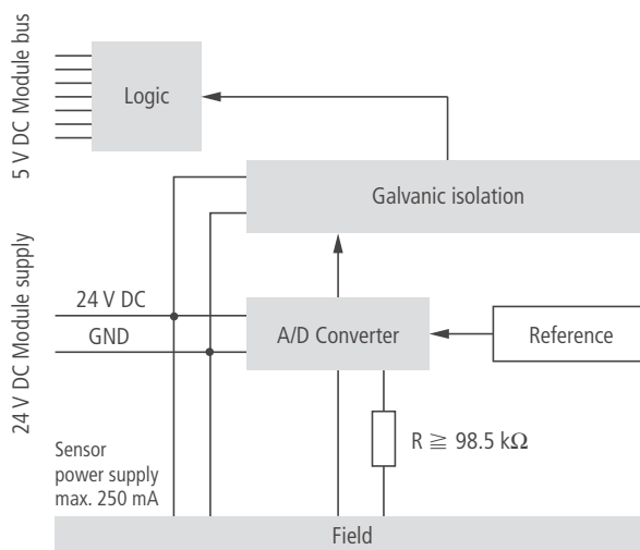
Figure 6-17: Block diagram
