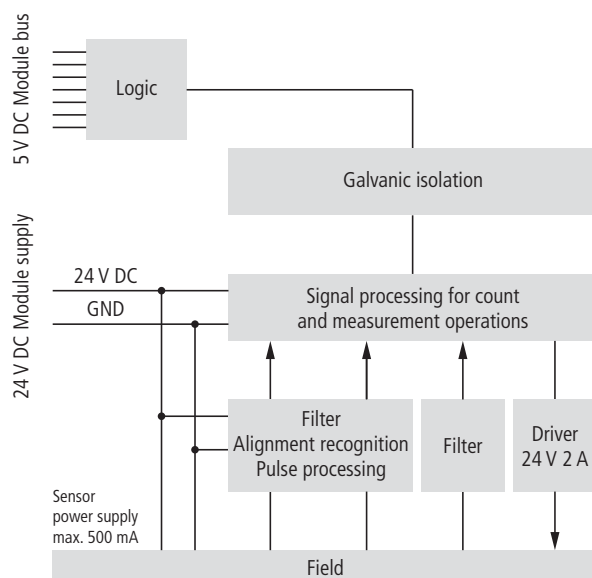
Figure 10-2: Block diagram
