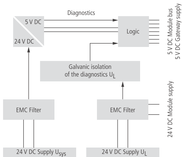
Figure 4-14: Block diagram
