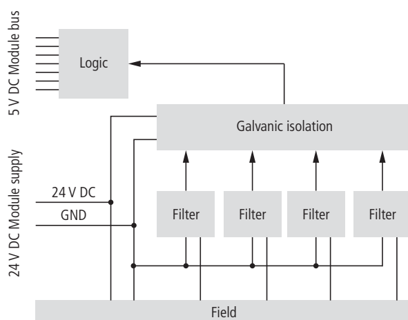
Figure 5-20: Block diagram
