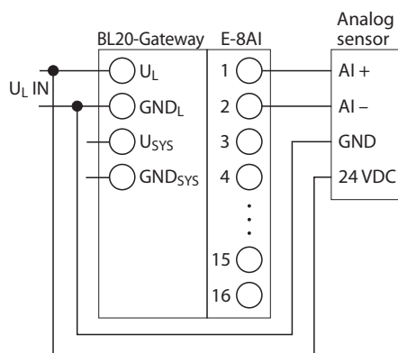
Figure 6-50: 4-wire-sensor (U/I)
