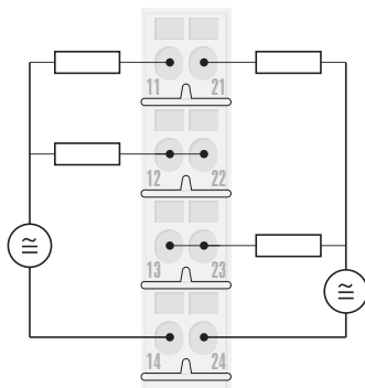
Figure 9-24: Wiring diagram BL20-S4x-SBBS
