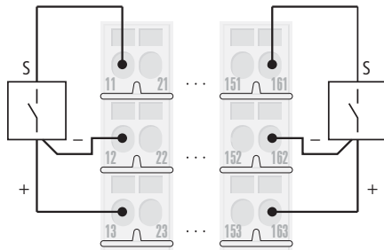
Figure 5-43: Wiring diagram BL20-B3×-SBB
