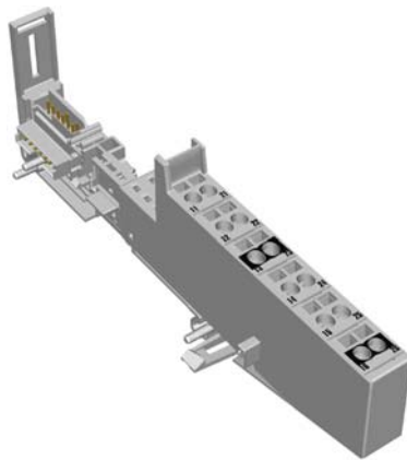
Figure 7-22: BL20-S6T-SBCSBC
