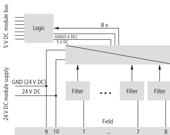
Figure 5-36: Block diagram
