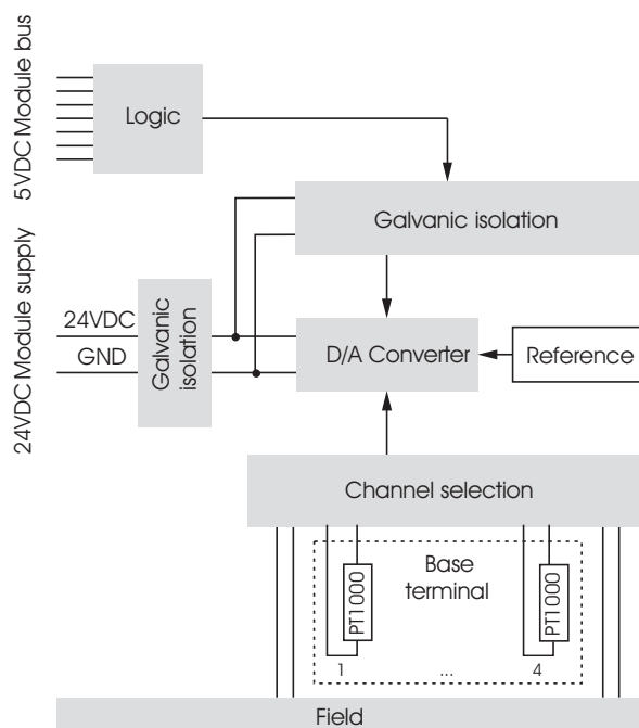
Figure 6-58: Block diagram
