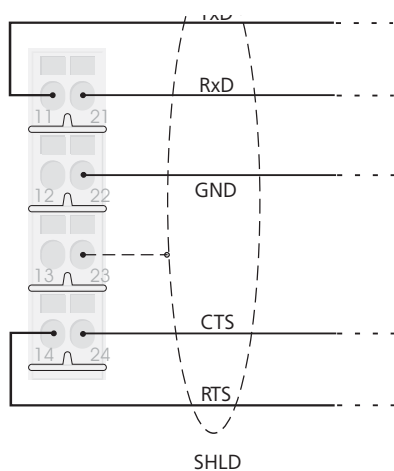
Figure 10-28: Wiring diagram BL20-S4x-SBBS
