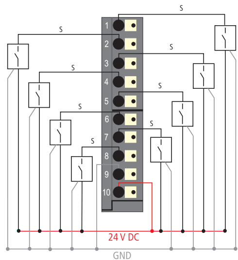
Figure 5-38: Wiring diagram with sensor supply
