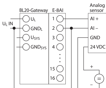
Figure 6-51: 4-wire-sensor (U/I)
