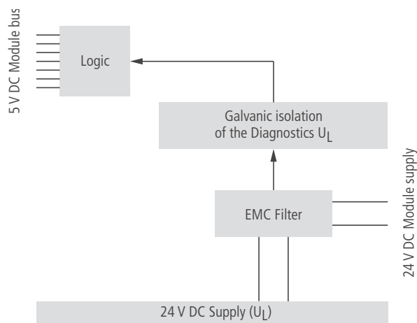
Figure 4-2: Block diagram
