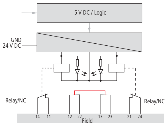
Figure 9-3: Block diagram with base module BL20-S4x-SBBS
