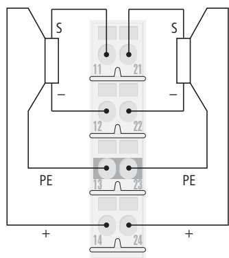
Figure 7-18: Wiring diagram BL20-S4x-SBCS
