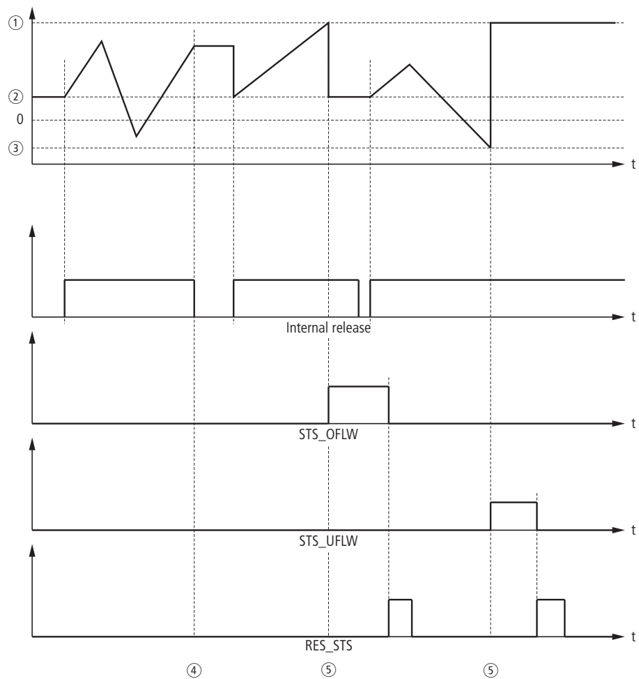
Figure 10-8: Single count with main count direc- tion down
