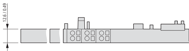
Figure 3-9: Base module in slice design (top view)
