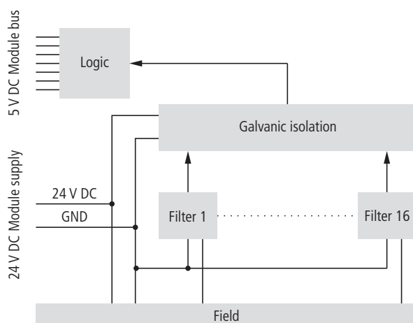
Figure 5-40: Block diagram
