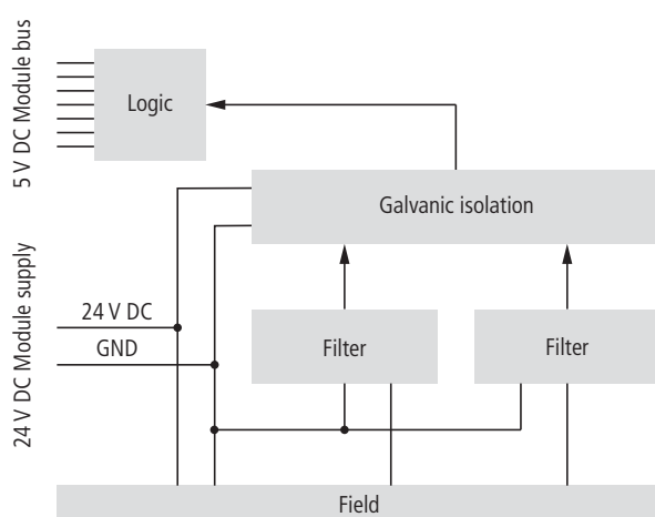
Figure 5-2: Block diagram
