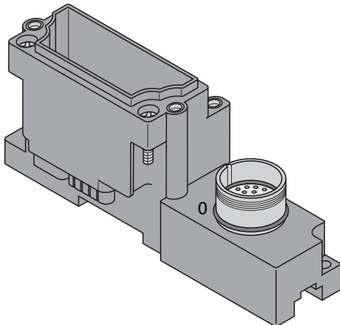
Figure 12-44: BL67-B-1M23
