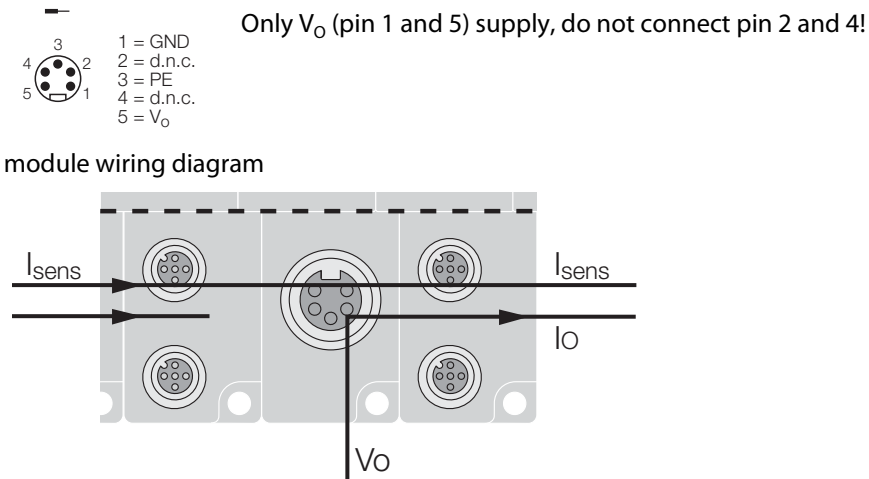
Figure 4-6: Pin assignment BL67-PF-24VDC with BL67-B-1RSM-VO
