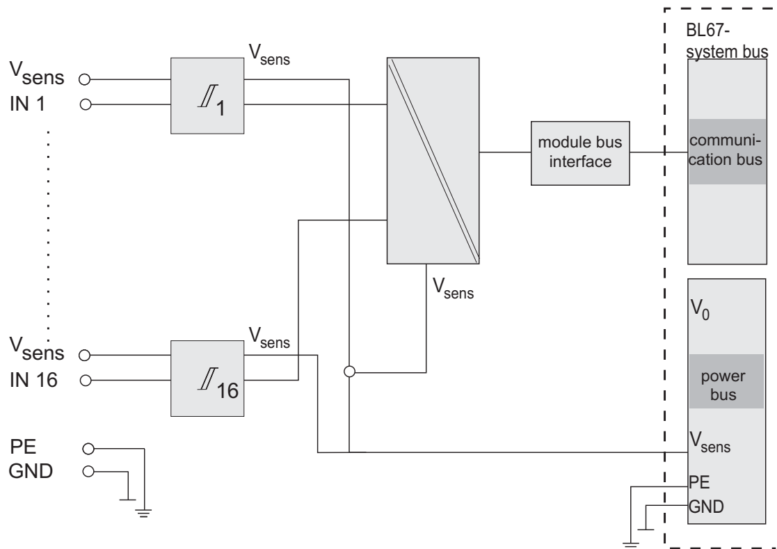
Figure 5-69: Block diagram
