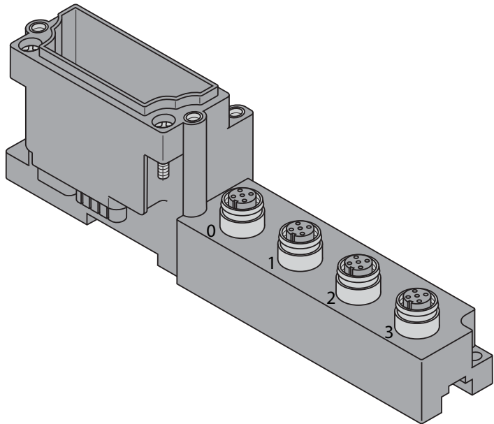
Figure 7-74: BL67-B-4M12/ BL67-B-4M12-P
