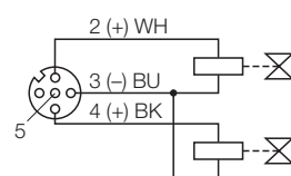
Figure 7-47: Wiring diagram BL67-8DO-0.5A-P with BL67-B-4M12
