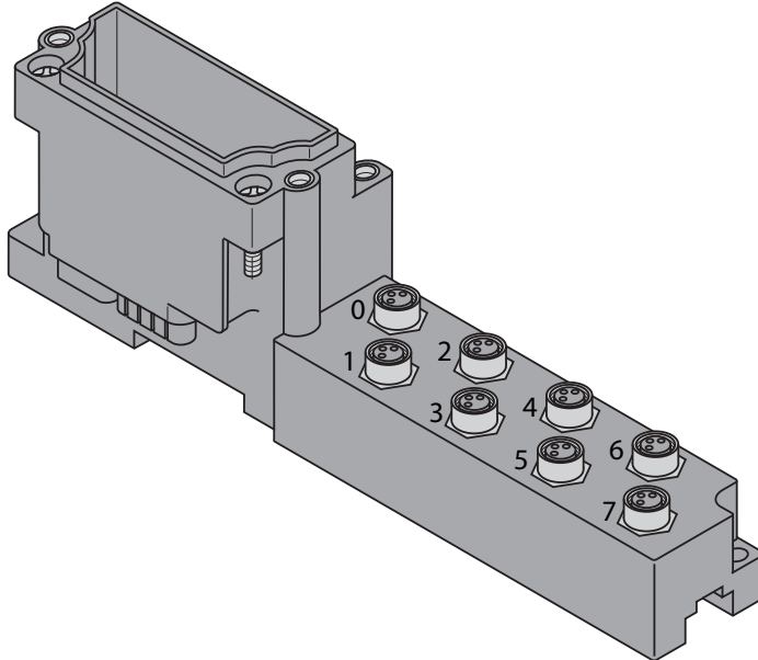
Figure 7-42: BL67-B-8M8
