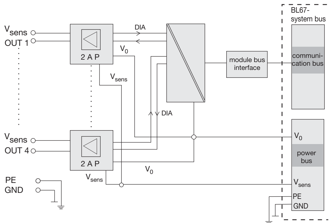
Figure 7-15: Block diagram
