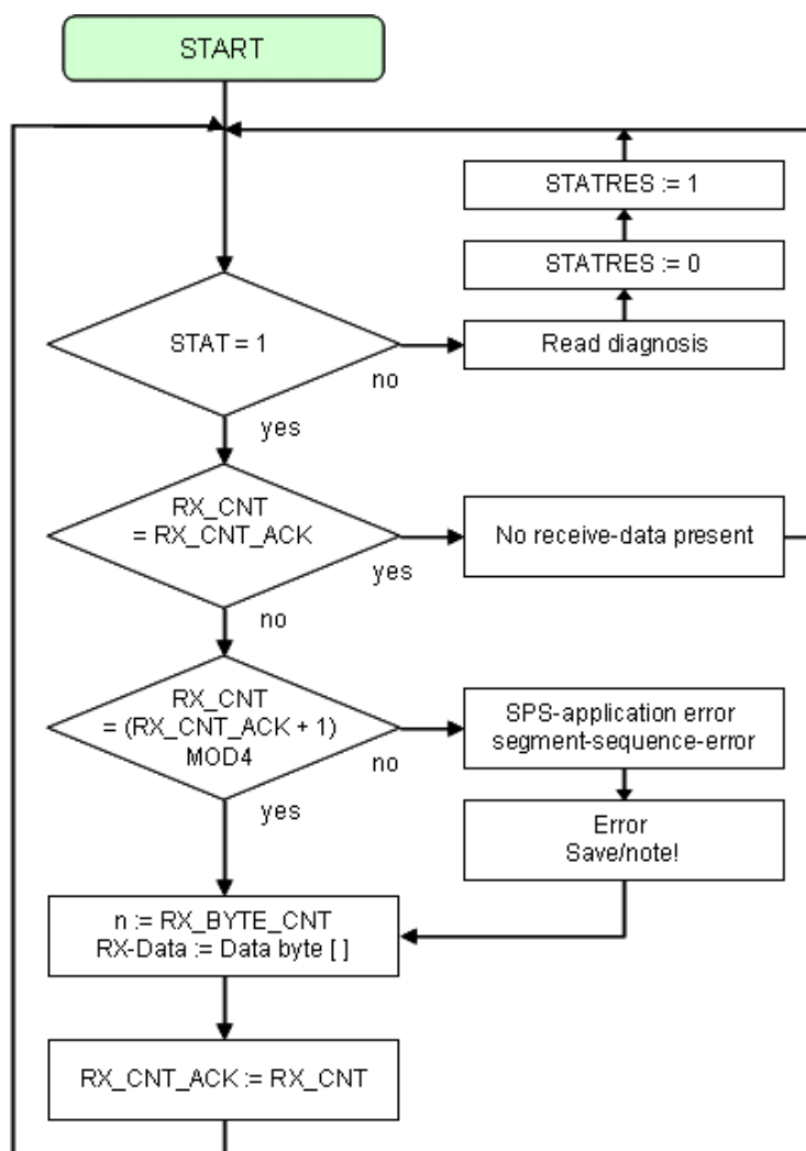
Figure 12-1: Schematic diagram of the receive sequence
