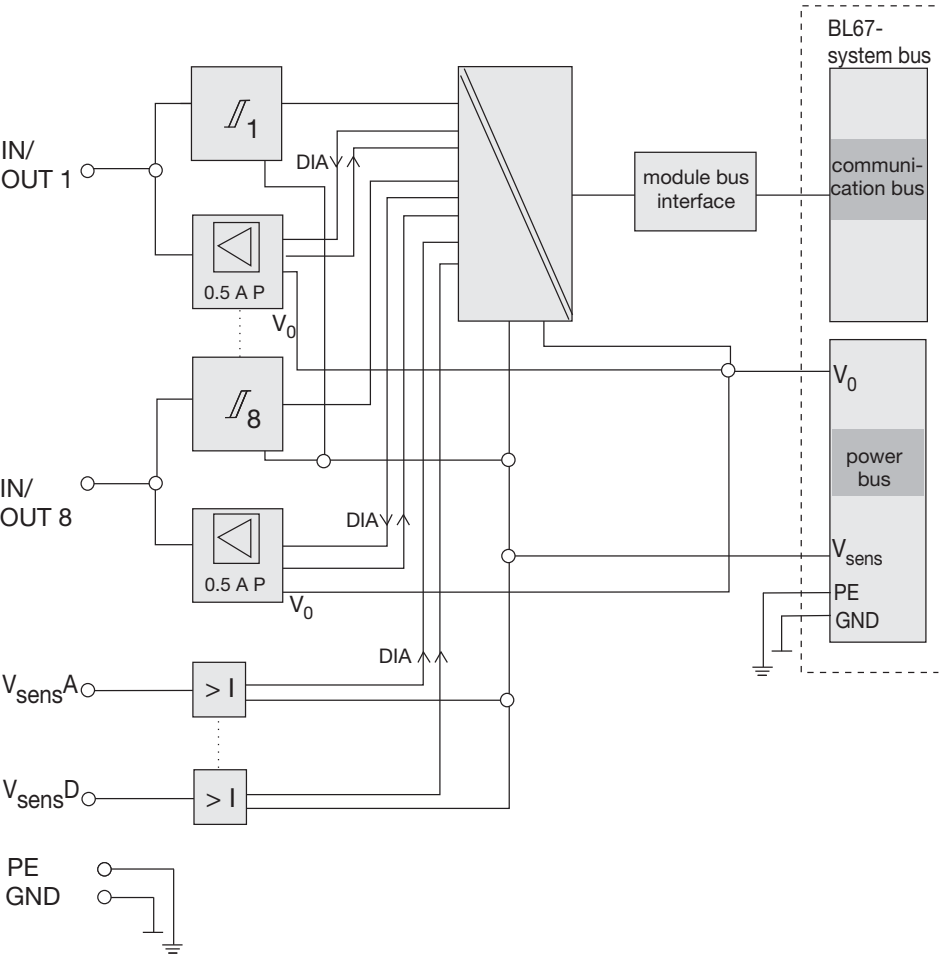
Figure 9-13: Block diagram
