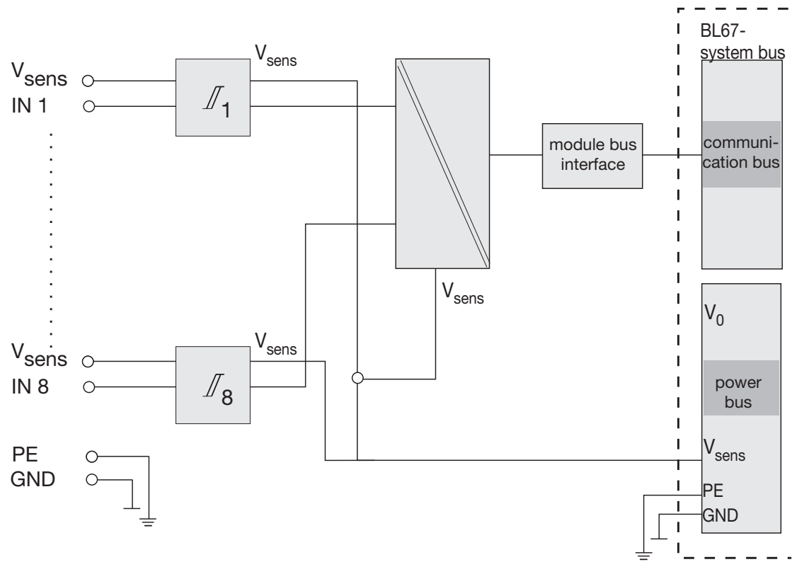
Figure 5-27: Block diagram
