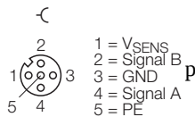
Figure 9-18: Pin assignment BL67-8XSG-PD with BL67-B- 4M12/BL67-B- 4M12-P
