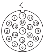
Figure 5-73: Pin assignment BL67-16DI-P with BL67-B-1M23-19
