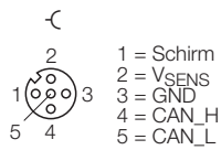
Figure 12-32: Pin assignment BL67-1CVI with BL67-B-1M12
