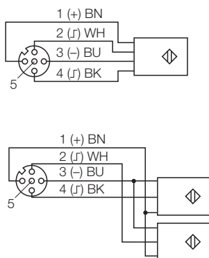
Figure 5-44: If the wire break detection has been activated, a jumper between pin 1 (24 VDC) and pin 2 (diagnostics input) must be implemented on the sensor side for monitoring of wire-breaks. Wiring diagram for wire break detection only with base module
