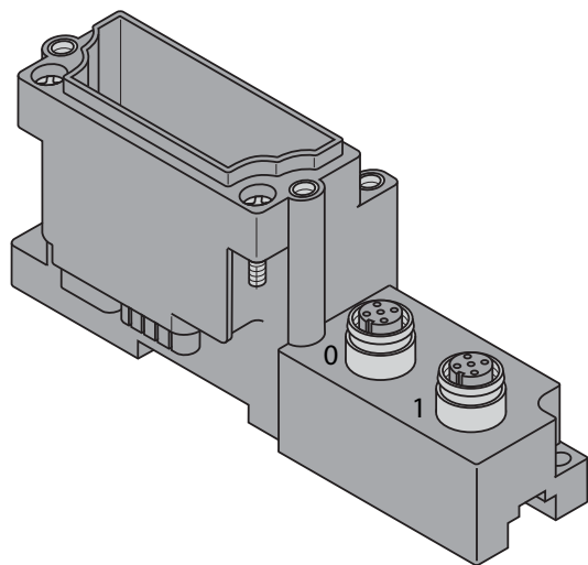
Figure 6-15: BL67-B-2M12
