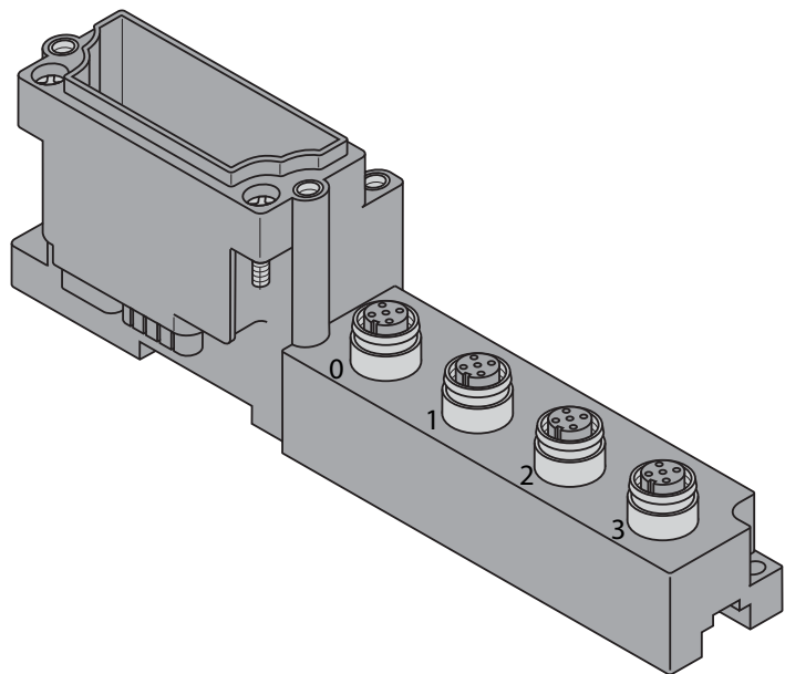
Figure 10-3: BL67-B-4M12
