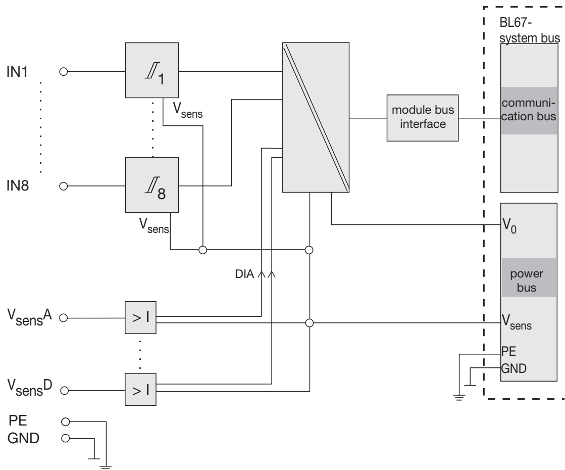
Figure 5-37: Block diagram
