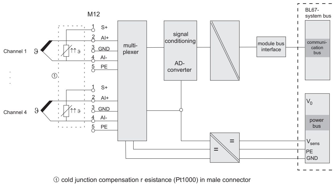
Figure 6-24: Block diagram
