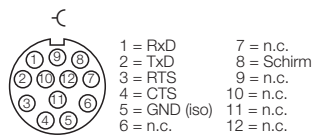
Figure 12-9: Pin assignment BL67-1RS232 with BL67-B-1M23
