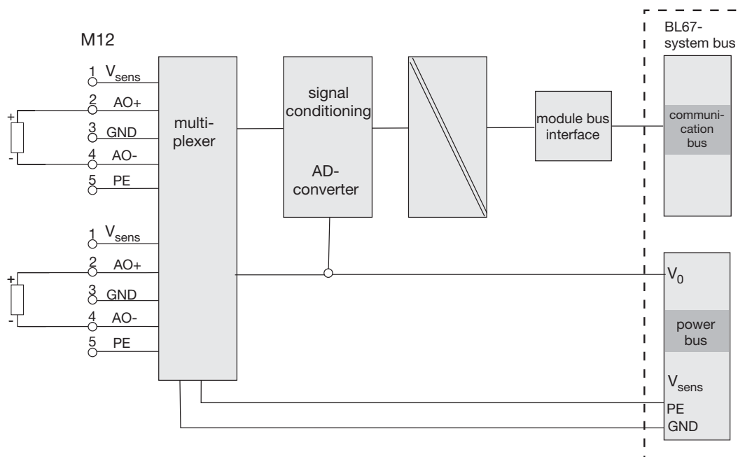
Figure 8-2: Block diagram
