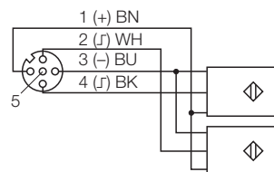
Figure 9-9: Wiring diagram BL67-4DI4DO-PD with BL67-B-4M12-P
