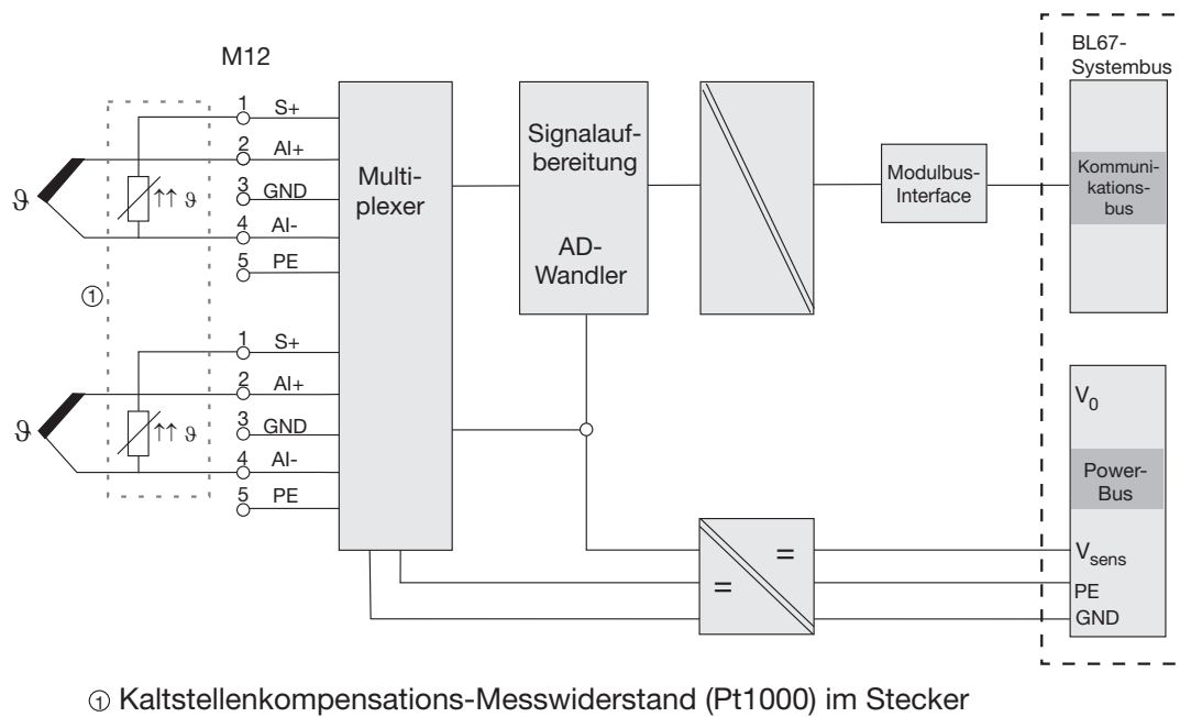
Figure 6-17: Block diagram
