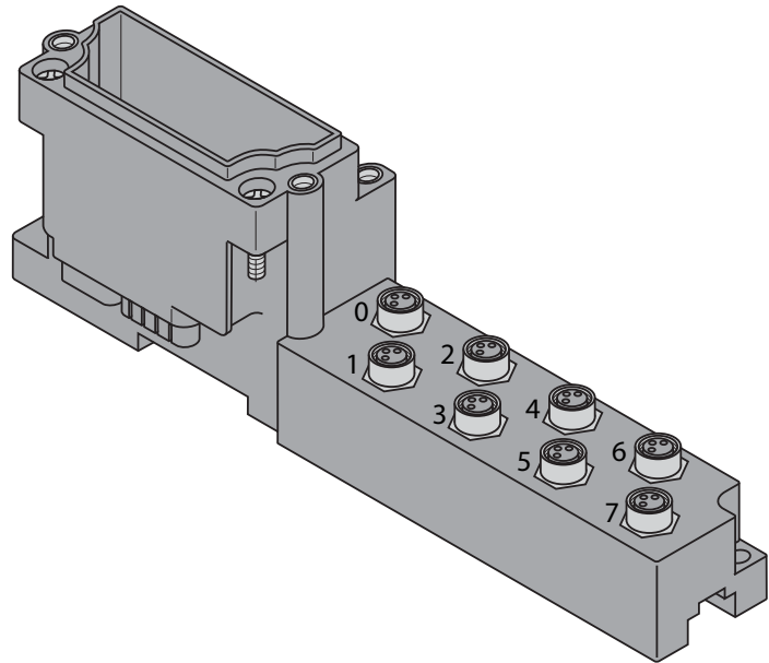
Figure 5-70: BL67-B-8M8-4-P
