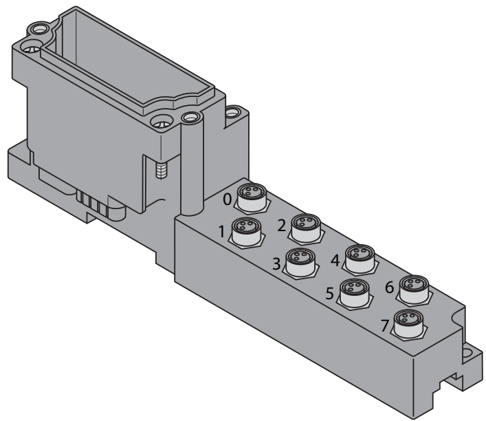
Figure 9-26: BL67-B-8M8
