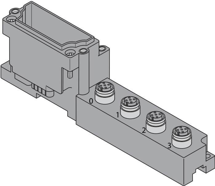
Figure 11-4: BL67-B-4M12
