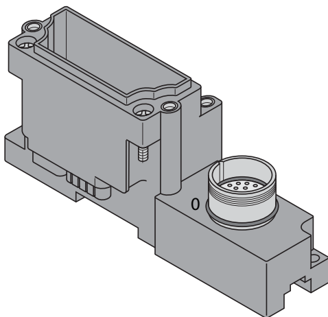
Figure 5-66: BL67-B-1M23
