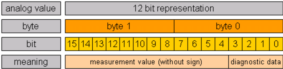
Figure 15-2: 12 bit representation
