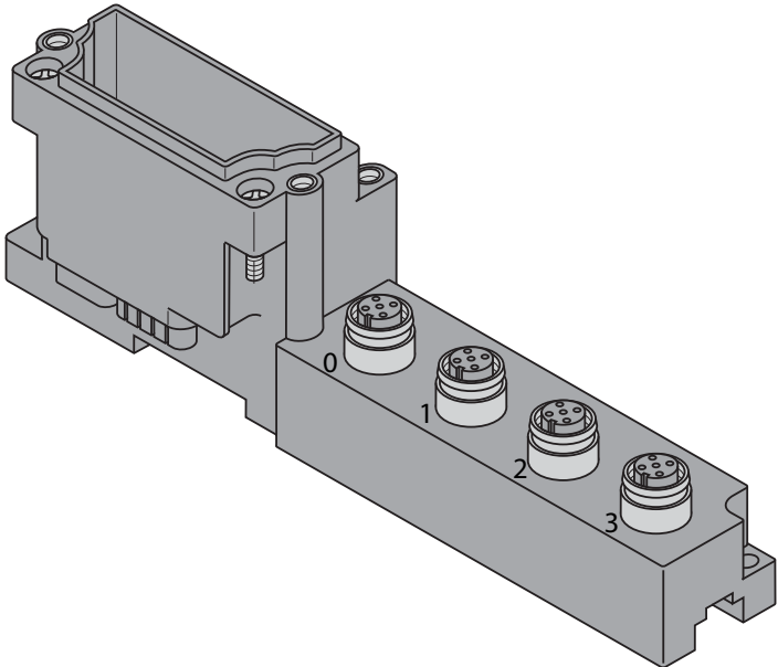
Figure 8-11: BL67-B-4M12
