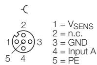
Figure 5-24: Pin assignment BL67-4DI-PD with BL67-B-4M12
