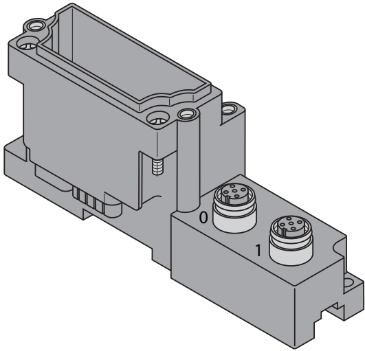
Figure 10-5: BL67-B-2M12/ BL67-B-2M12-8-P
