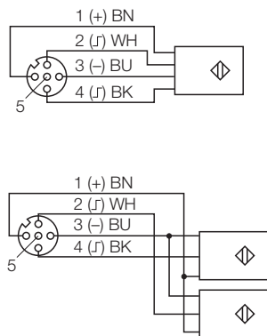
Figure 5-52: Wiring diagram BL67-4DI-N with BL67-B-2M12/ BL67-B-2M12-P
