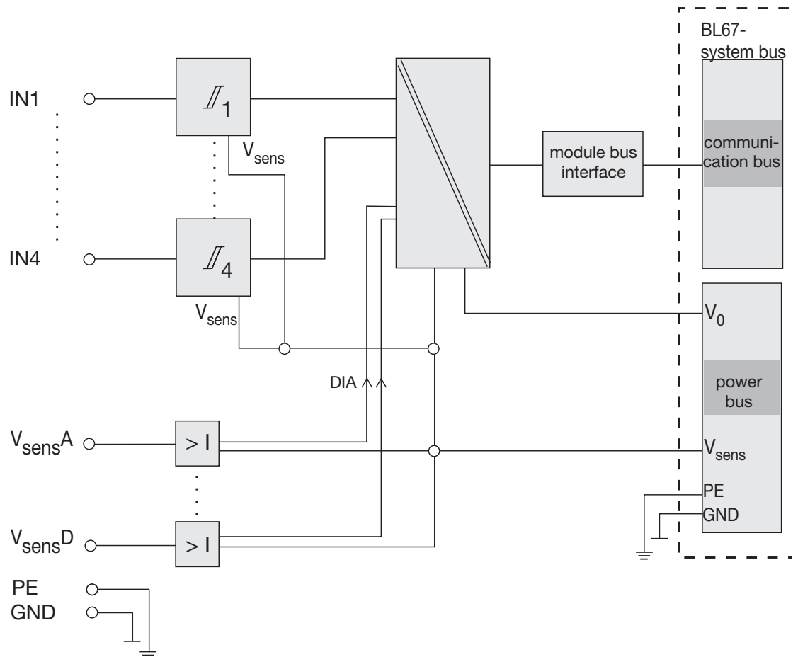
Figure 5-15: Block diagram
