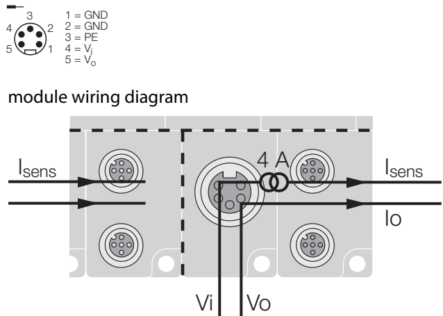
Figure 4-4: Pin assignment BL67-PF-24VDC with BL67-B-1RSM
