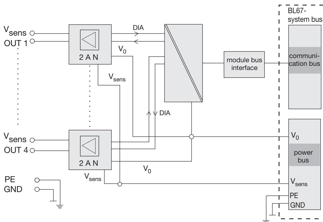
Figure 7-57: Block diagram
