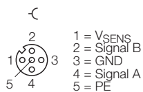
Figure 9-7: Pin assignment BL67-4DI4DO-PD with BL67-B-4M12/ BL67-B-4M12-P
