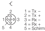
Figure 12-16: pin assignment BL67-1RS485/422 with BL67-B-1M12
