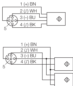
Figure 5-8: Wiring diagram BL67-4DI-P with BL67-B-2M12/ BL67-B-2M12-P
