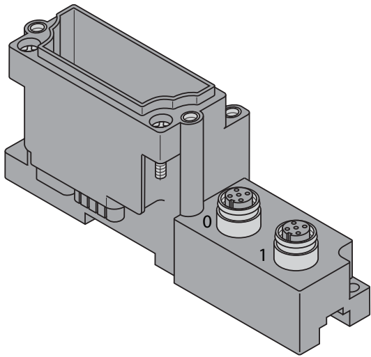
Figure 7-32: BL67-B-2M12/ BL67-B-2M12-P
