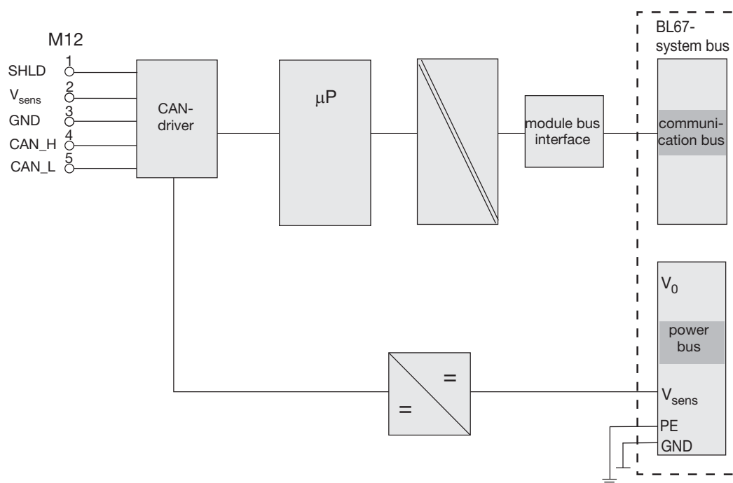
Figure 12-30: Block diagram BL67-1CVI
