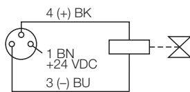
Figure 7-18: Wiring diagram BL67-4DO-2A-P with BL67-B-4M8
