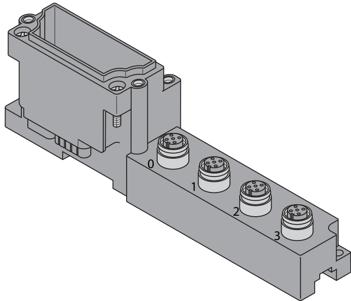
Figure 7-45: BL67-B-4M12/ BL67-B-4M12-P
