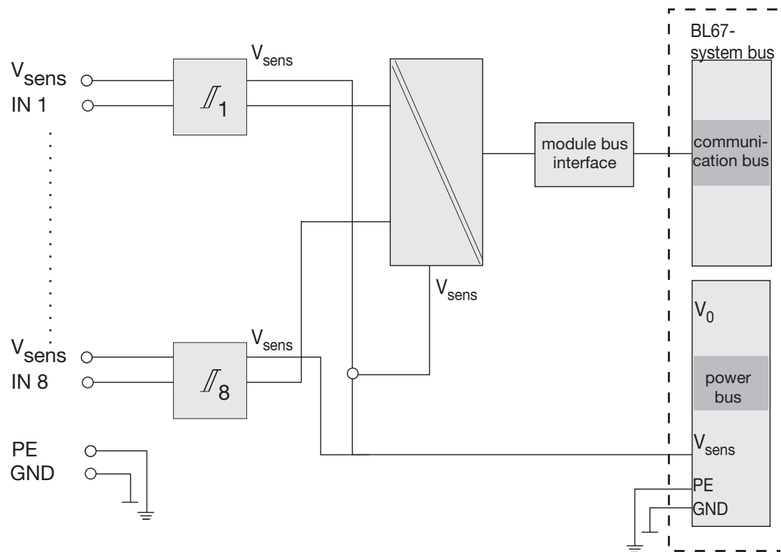
Figure 5-59: Block diagram
