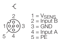
Figure 5-42: Pin assignment BL67-8DI-PD with BL67-B-4M12/ BL67-B-4M12-P
