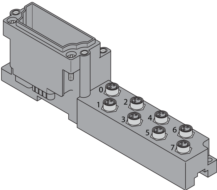
Figure 7-54: BL67-B-8M8-4-P
