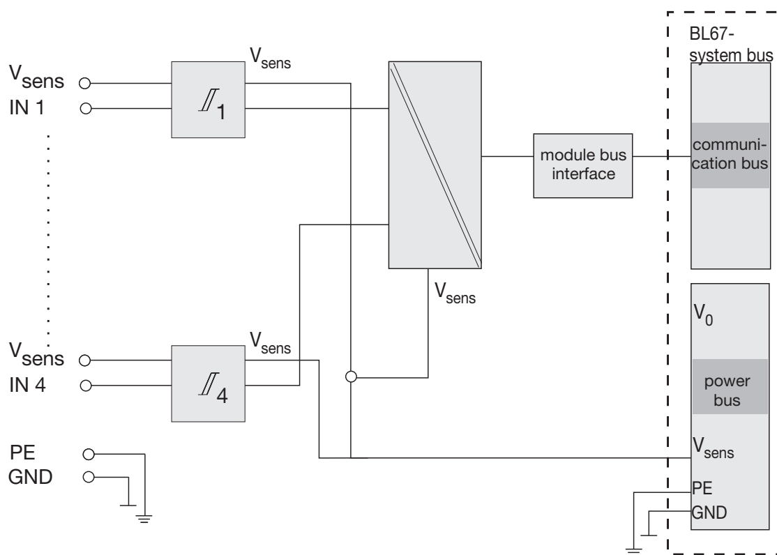
Figure 5-2: Block diagram
