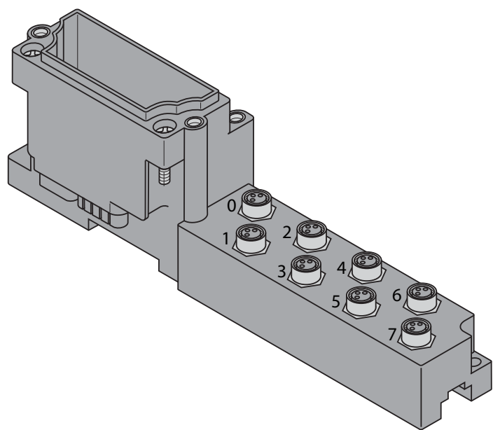
Figure 10-6: BL67-B-8M8
