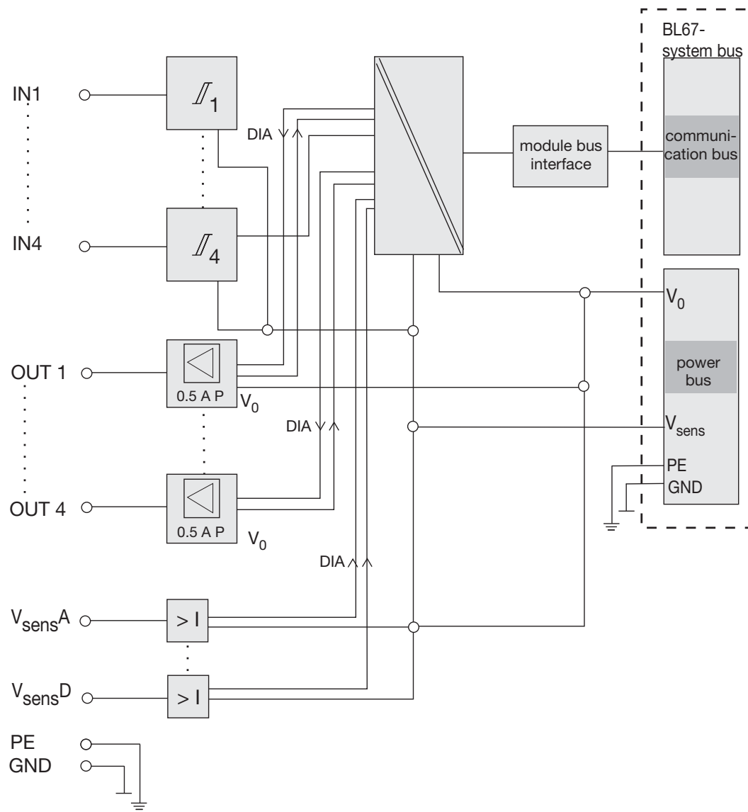
Figure 9-2: Block diagram
