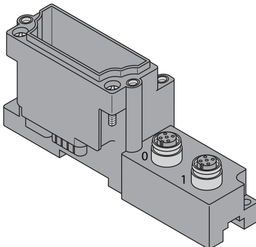
Figure 5-6: BL67-B-2M12/ BL67-B-2M12-P
