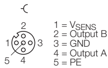
Figure 7-75: Pin assignment BL67-8DO-0.5A-N with BL67-B-4M12
