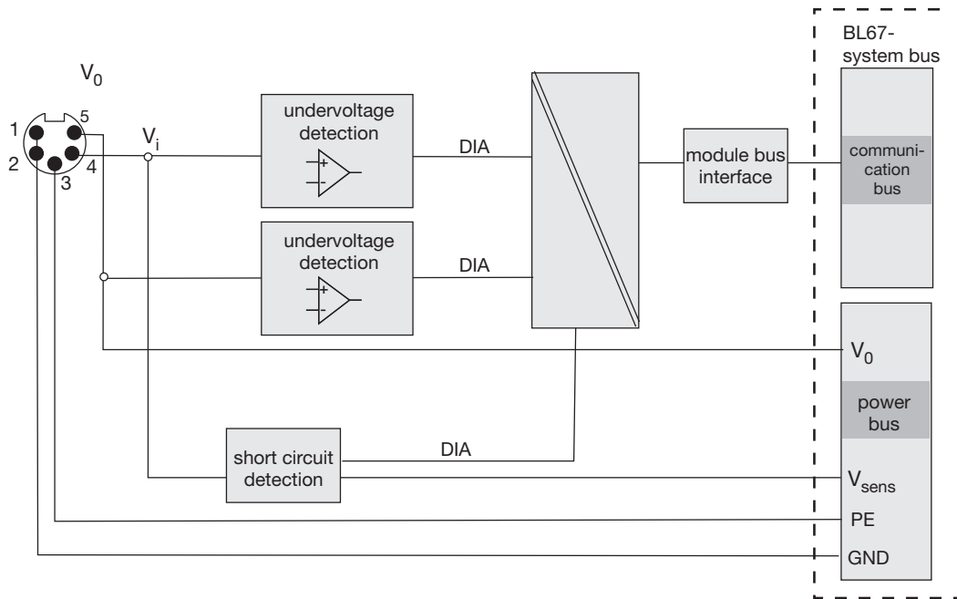
Figure 4-2: Block diagram
