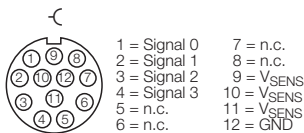
Figure 7-68: Pin assignment BL67-4DO-2A-N with BL67-B-1M23
