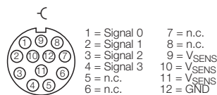
Figure 5-13: Pin assignment BL67-4DI-P with BL67-B-1M23
