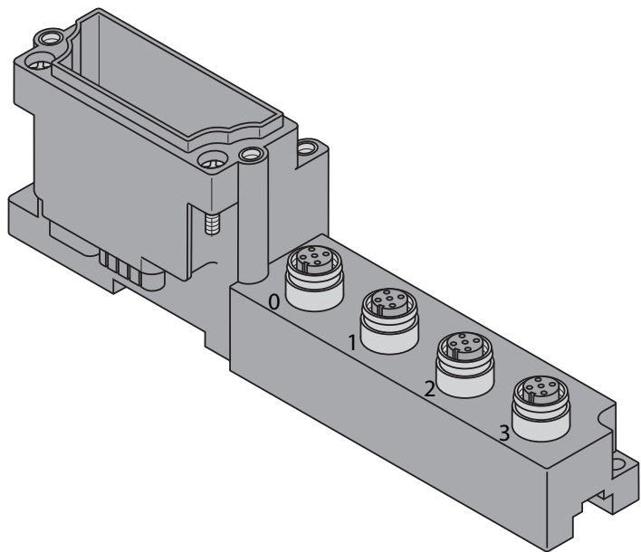
Figure 5-9: BL67-B-4M12
