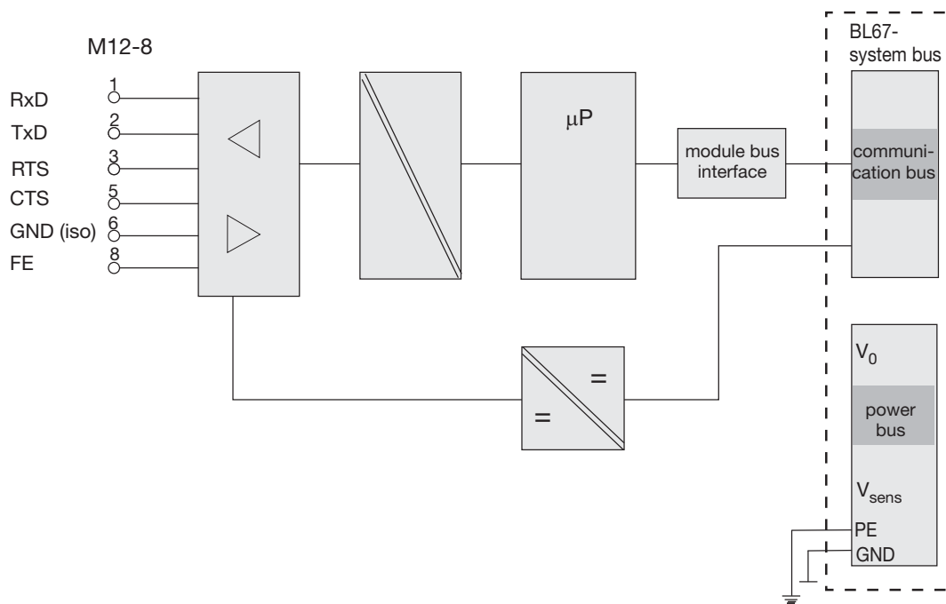
Figure 12-4: Block diagram
