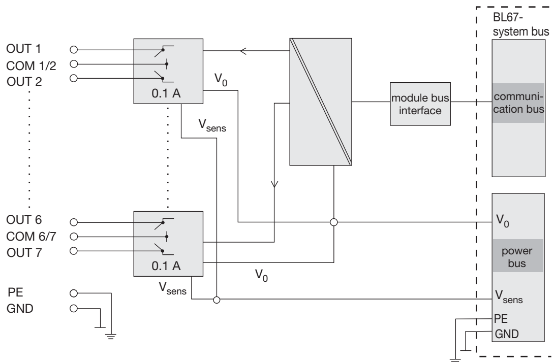
Figure 11-3: Block diagram
