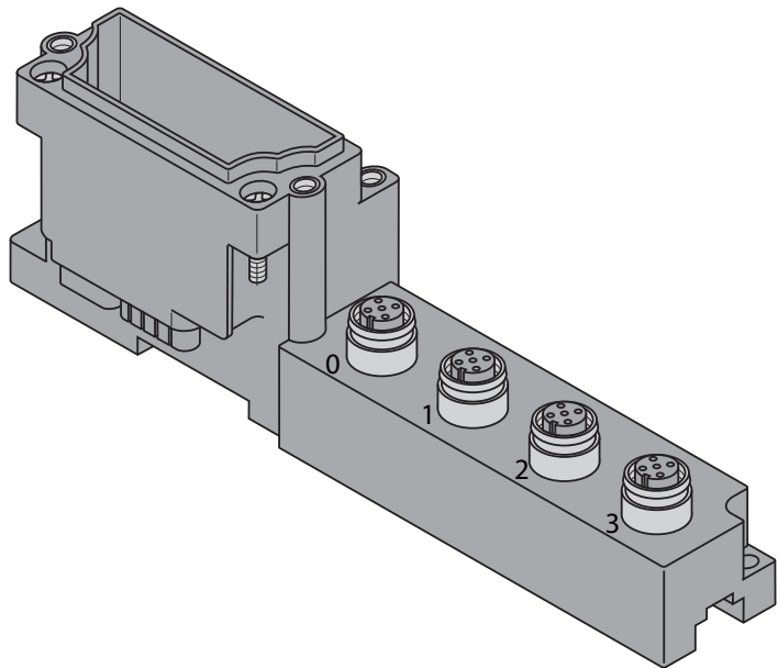
Figure 7-35: BL67-B-4M12
