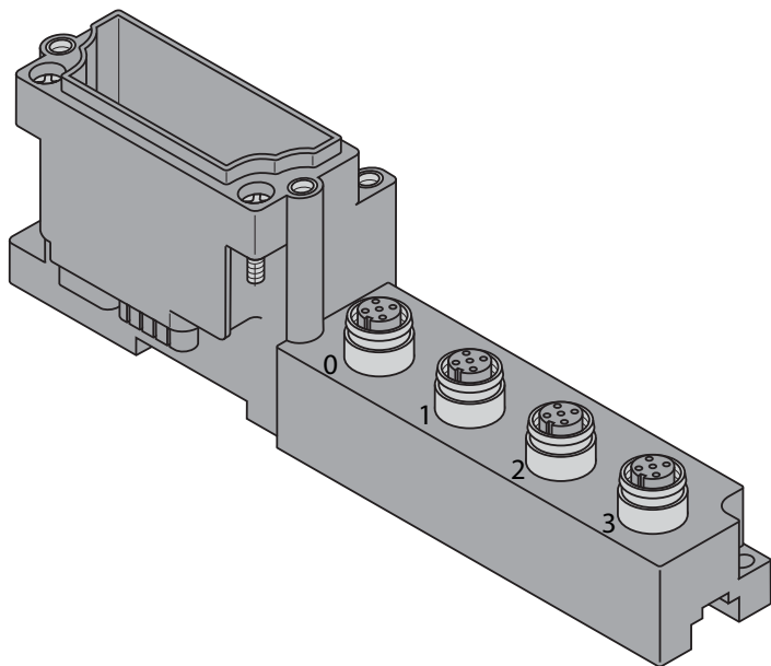
Figure 6-21: BL67-B-4M12
