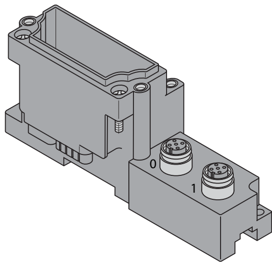
Figure 5-50: BL67-B-2M12/ BL67-B-2M12-P
