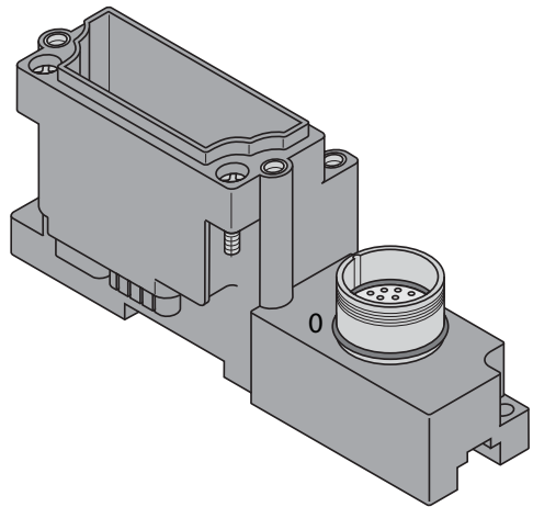
Figure 7-25: BL67-B-1M23
