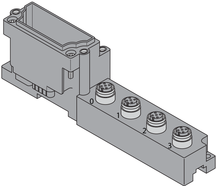
Figure 5-31: BL67-B-4M12/ BL67-B-4M12-P
