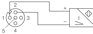
Figure 6-8: Wiring diagrams BL67-2AI-I
