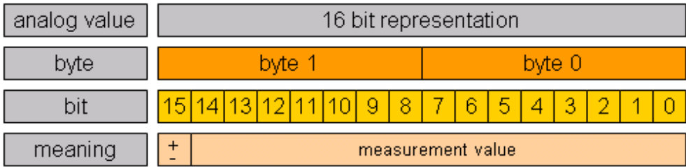
Figure 6-1: 16-bit-representation
