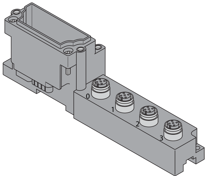
Figure 5-63: BL67-B-4M12/ BL67-B-4M12-P
