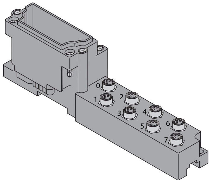
Figure 5-28: BL67-B-8M8
