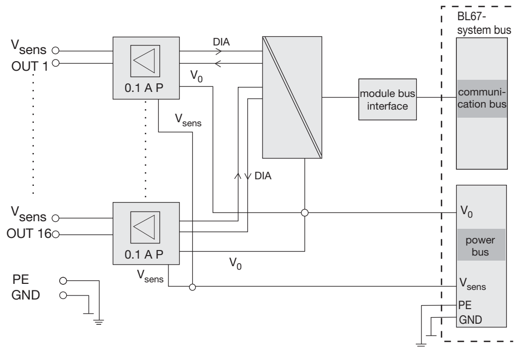
Figure 7-51: Block diagram
