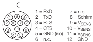
Figure 12-10: Pin assignment BL67-1RS232 with BL67-1M23-VI
