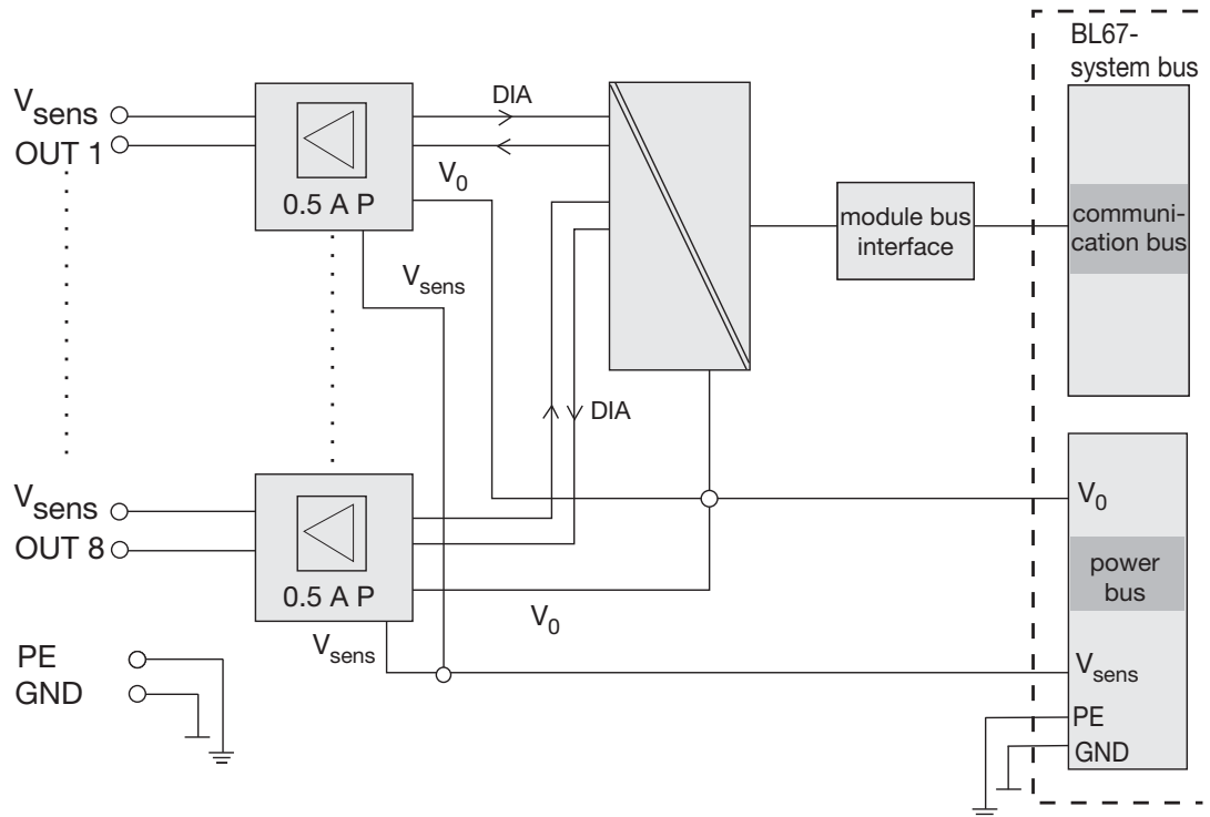
Figure 7-41: Block diagram
