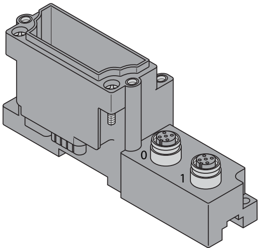
Figure 8-12: BL67-B-2M12/ BL67-B-2M12-8-P
