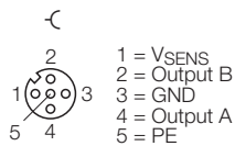
Figure 7-33: Pin assignment BL67-4DO-4A-P with BL67-B-2M12/ BL67-B-2M12-P
