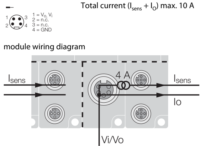
Figure 4-5: Pin assignment BL67-PF-24VDC with BL67-B-1RSM-4
