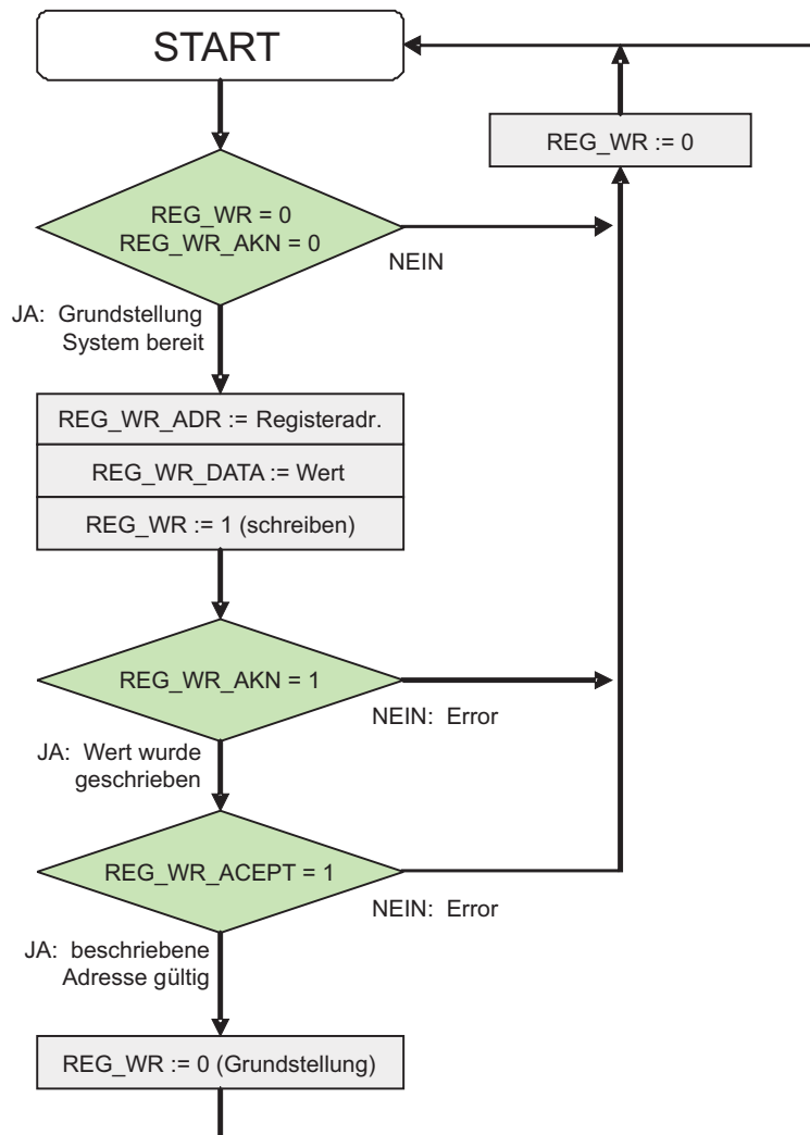
Figure 12-48: Schematic diagram of the write sequence
