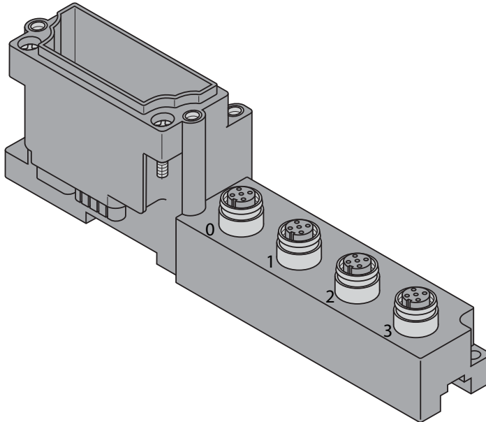
Figure 6-25: BL67-B-4M12
