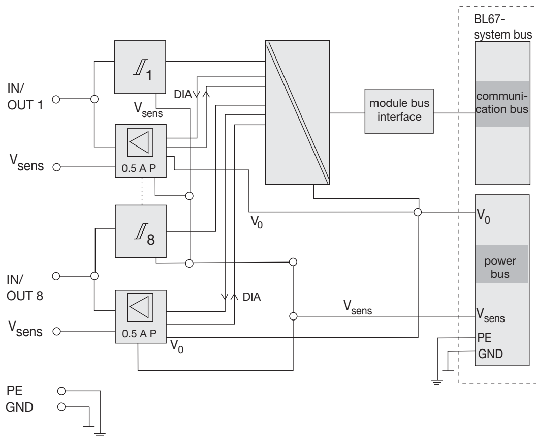
Figure 9-25: Block diagram
