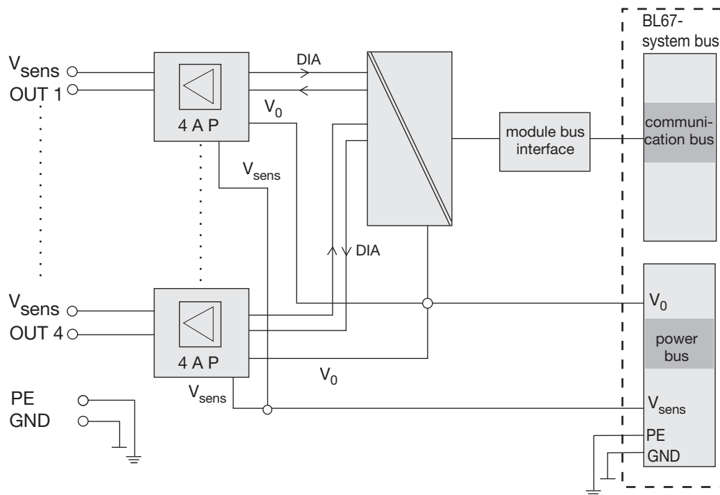
Figure 7-28: Block diagram
