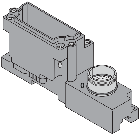
Figure 5-72: BL67-B-1M23-19
