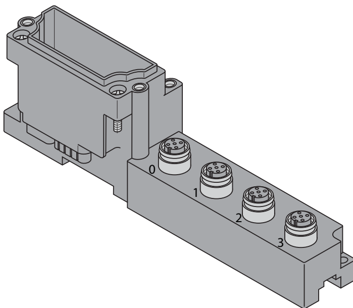
Figure 5-41: BL67-B-4M12/ BL67-B-4M12-P
