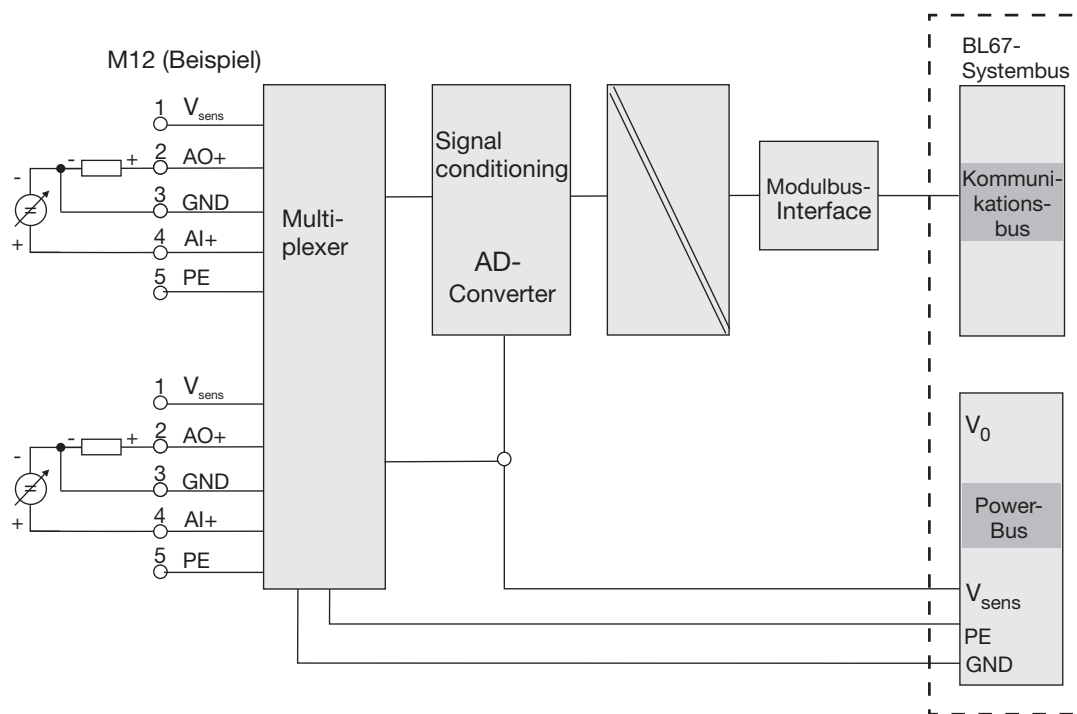
Figure 10-2: Block diagram
