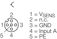
Figure 5-54: Pin assignment BL67-4DI-N with BL67-B-4M12
