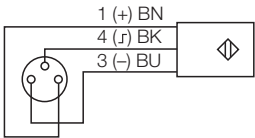
Figure 9-5: Wiring diagram BL67-4DI4DO-PD with BL67-B-8M8
