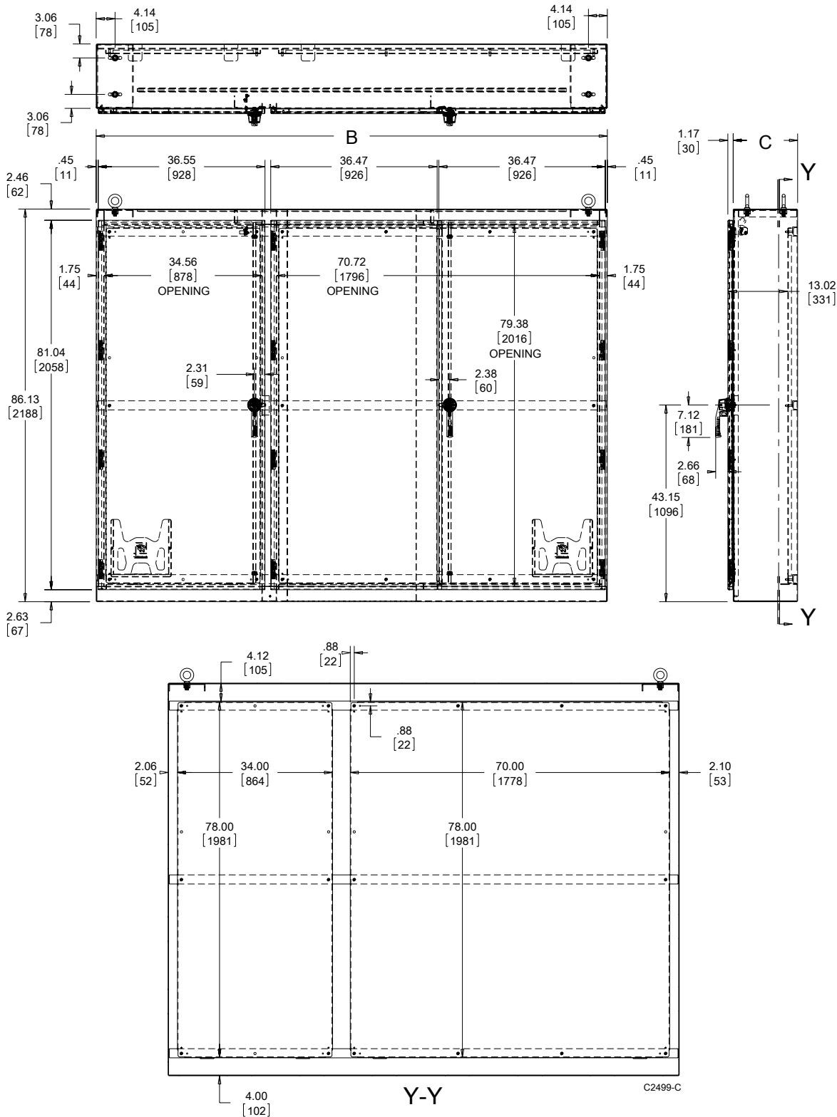
Three-Door Enclosure
