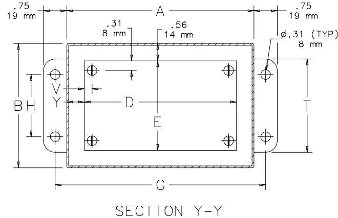
SECTION Y-Y
