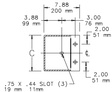
SECTION W-W
