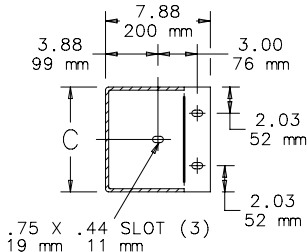
SECTION W-W
