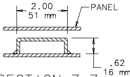
SECTION Z-Z
