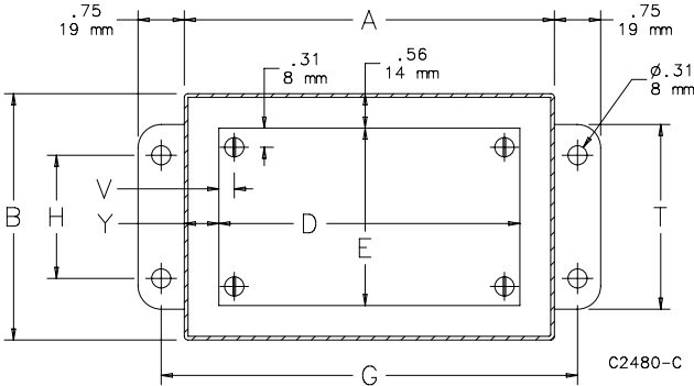
SECTION Y-Y
