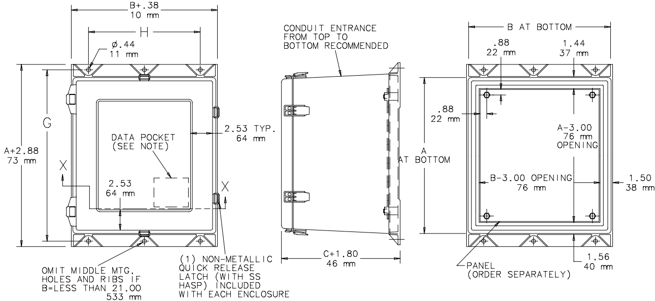
Hinged with Quick-Release Latch Enclosures 36 X 30 or Smaller Drawing
