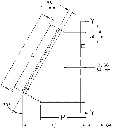
VIEW X-X
