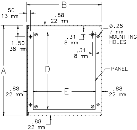
SECTION Y-Y
