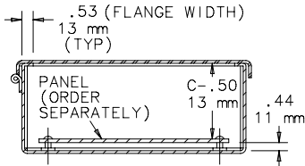
SECTION X-X
