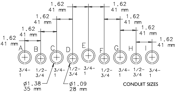
Knockout Pattern (from outside of box)
