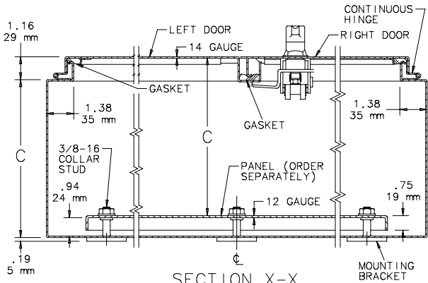
SECTION X-X
