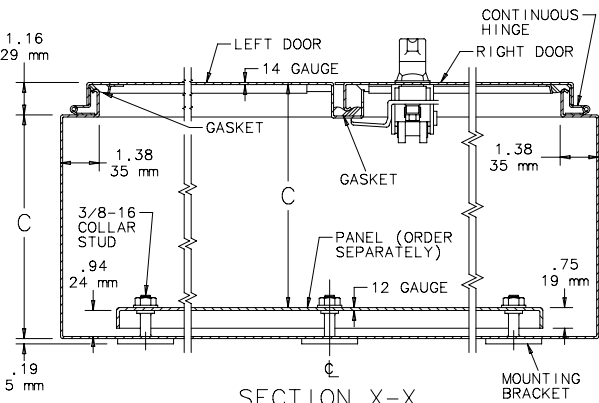
SECTION X-X
