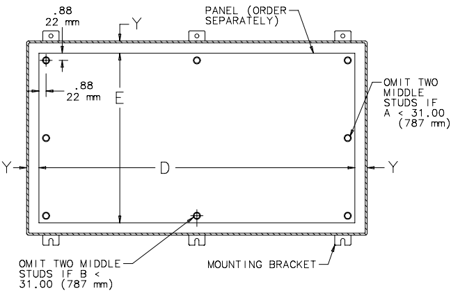
SECTION Y-Y
