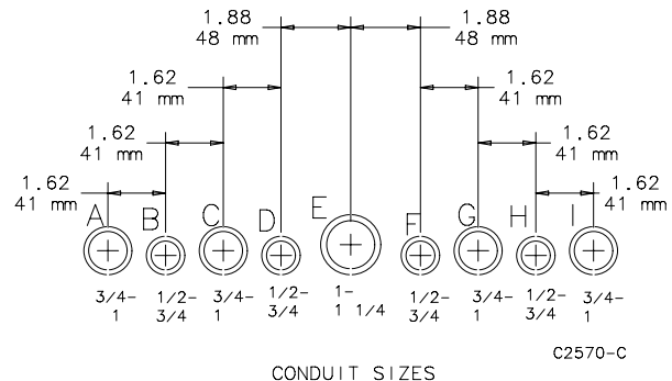
CONDUIT SIZES Knockout Pattern (from outside of box)
